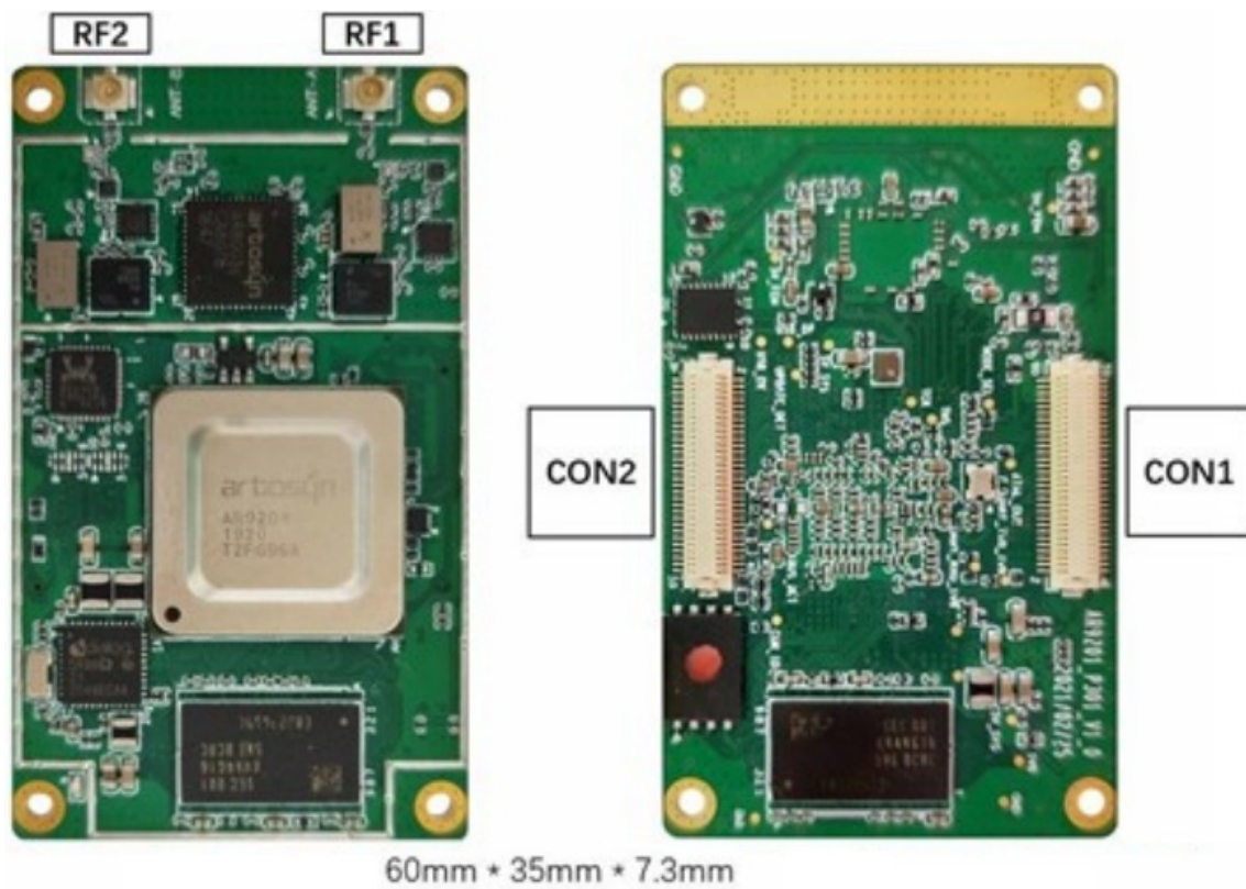
Front Figure-2: P301-D Module Back
