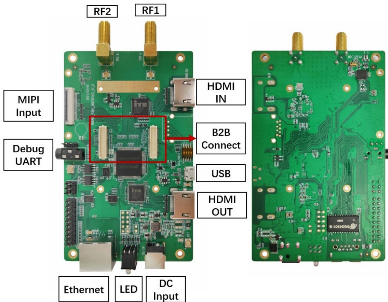
Front Figure-3: P301-D EVB Board Back
