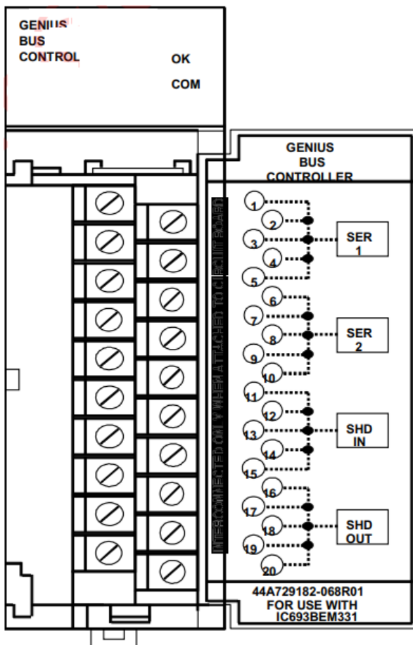
Figure 8-5. Genius Bus Controller Module
