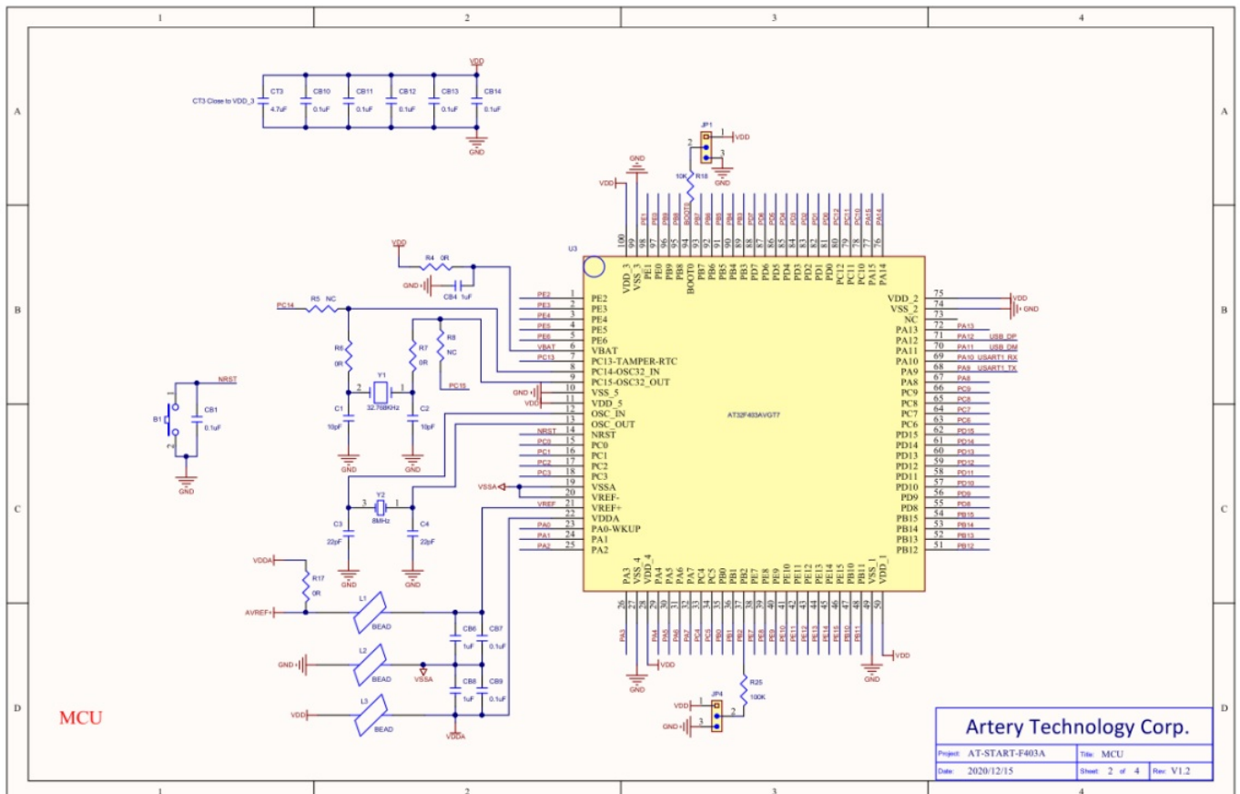
Figure 5. Schematic (microcontroller)
