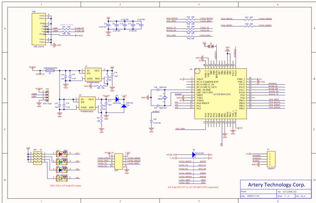
Figure 4. Schematic (AT-Link-EZ)
