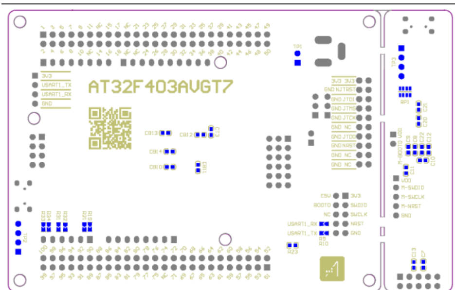
Figure 3. Bottom layer
