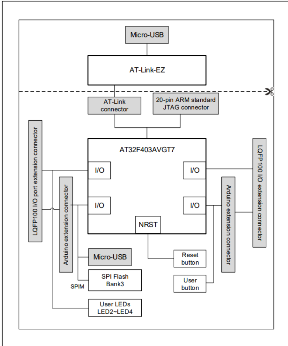
Figure 1. Hardware block diagram
