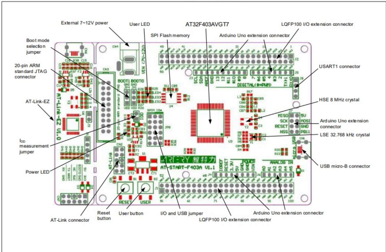
Figure 2. Top layer
