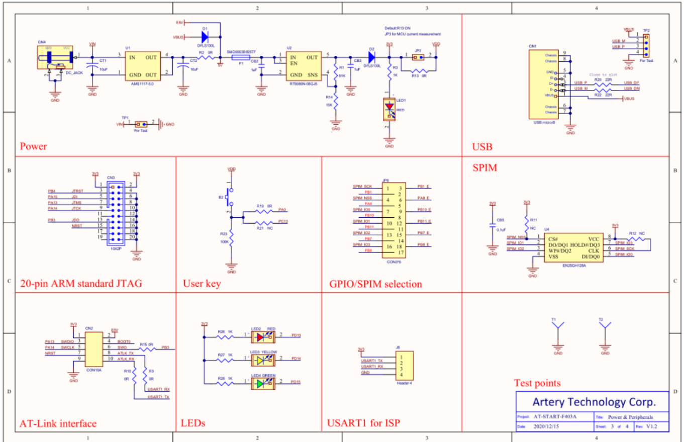
Figure 6. Schematic (power supply and peripherals)
