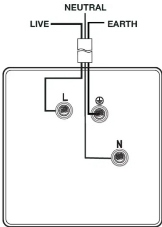
13AMP 2 GANG SWITCHED SOCKET
