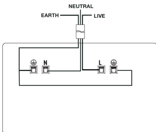
13AMP 2 GANG SWITCHED SOCKET WITH US
