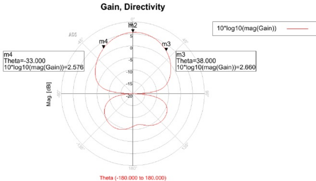
Fig. 7 Antenna Gain over X-Z plane
