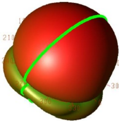
Fig. 8 Antenna Diagram and Y-Z plane cut
