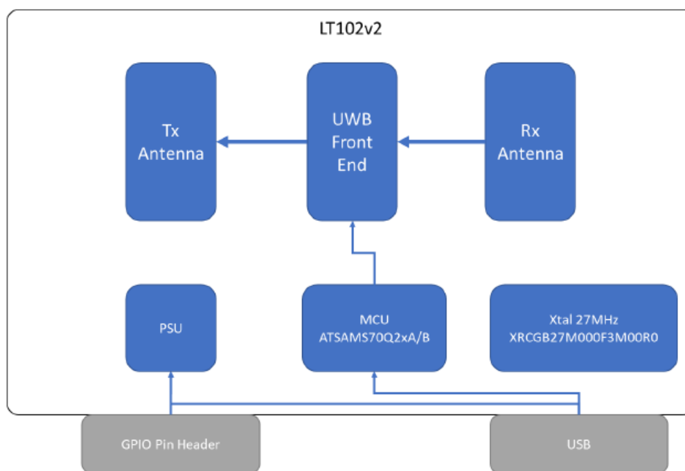
Fig. 2 LT102v2 System Diagram
