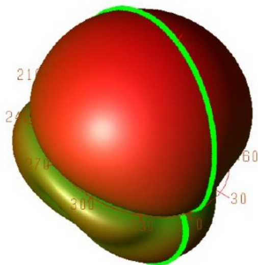
Fig. 5 Antenna Diagram and X-Z plane cut
