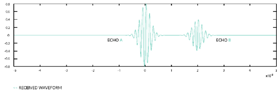
Fig. 1: The basic principle and the waveforms
