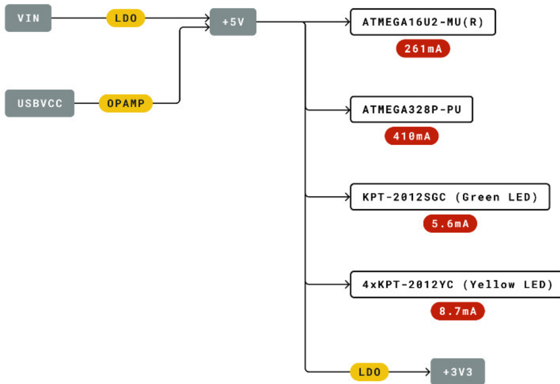
Power tree
