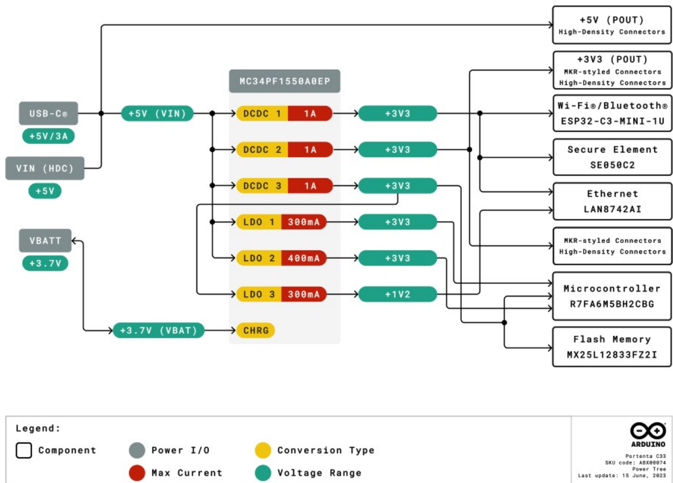
Figure 4. Power architecture of the Portenta C33
