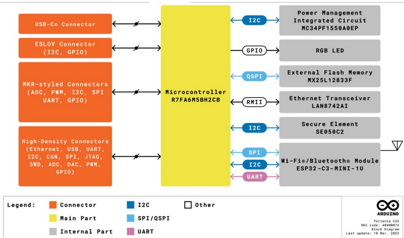
Figure 3. High-level architecture of the Portenta C33
