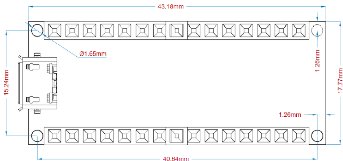
Mechanical dimensions of Arduino Nano RP2040 Connect
