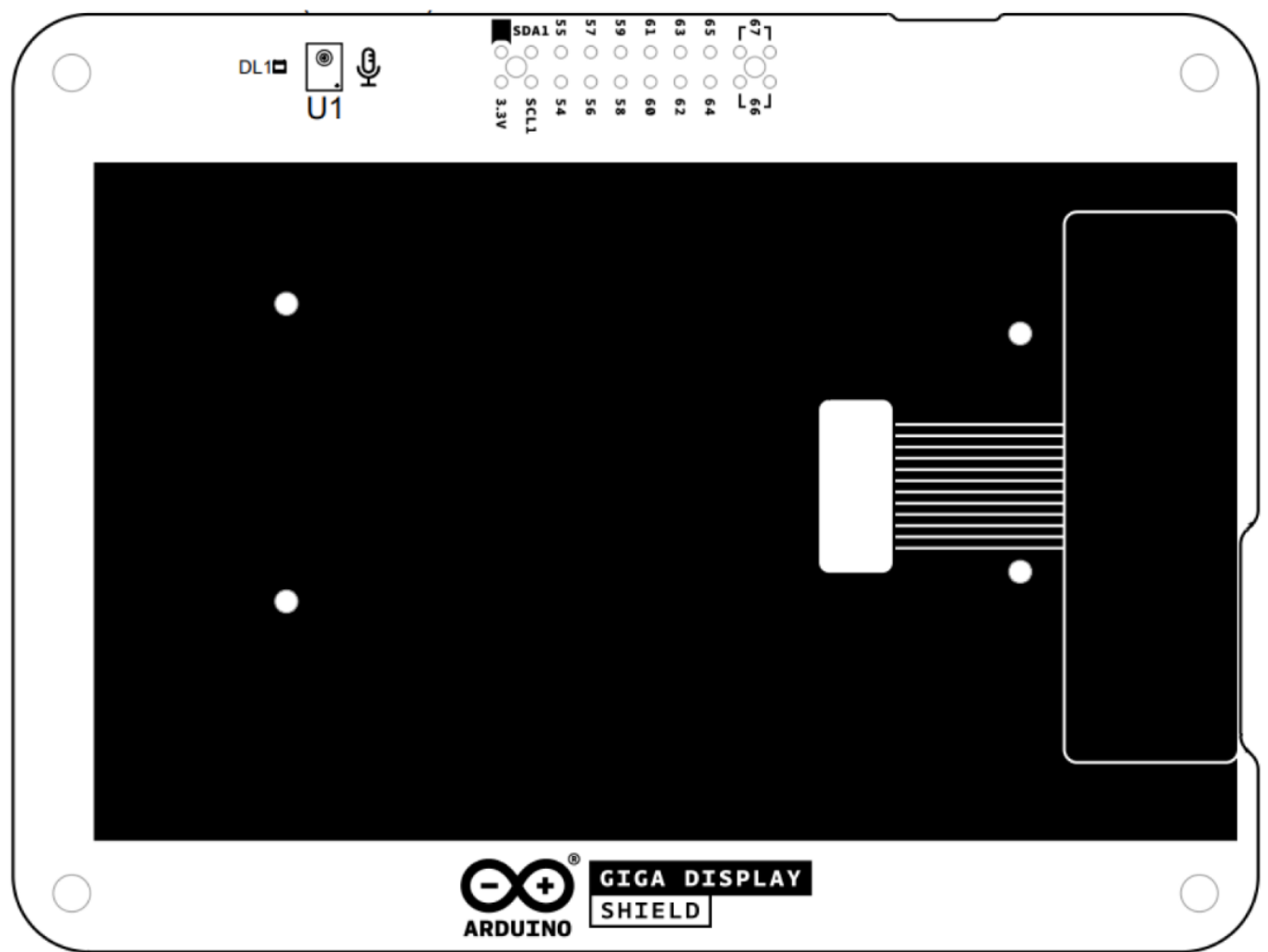
Top View of Arduino GIGA Display Shield
