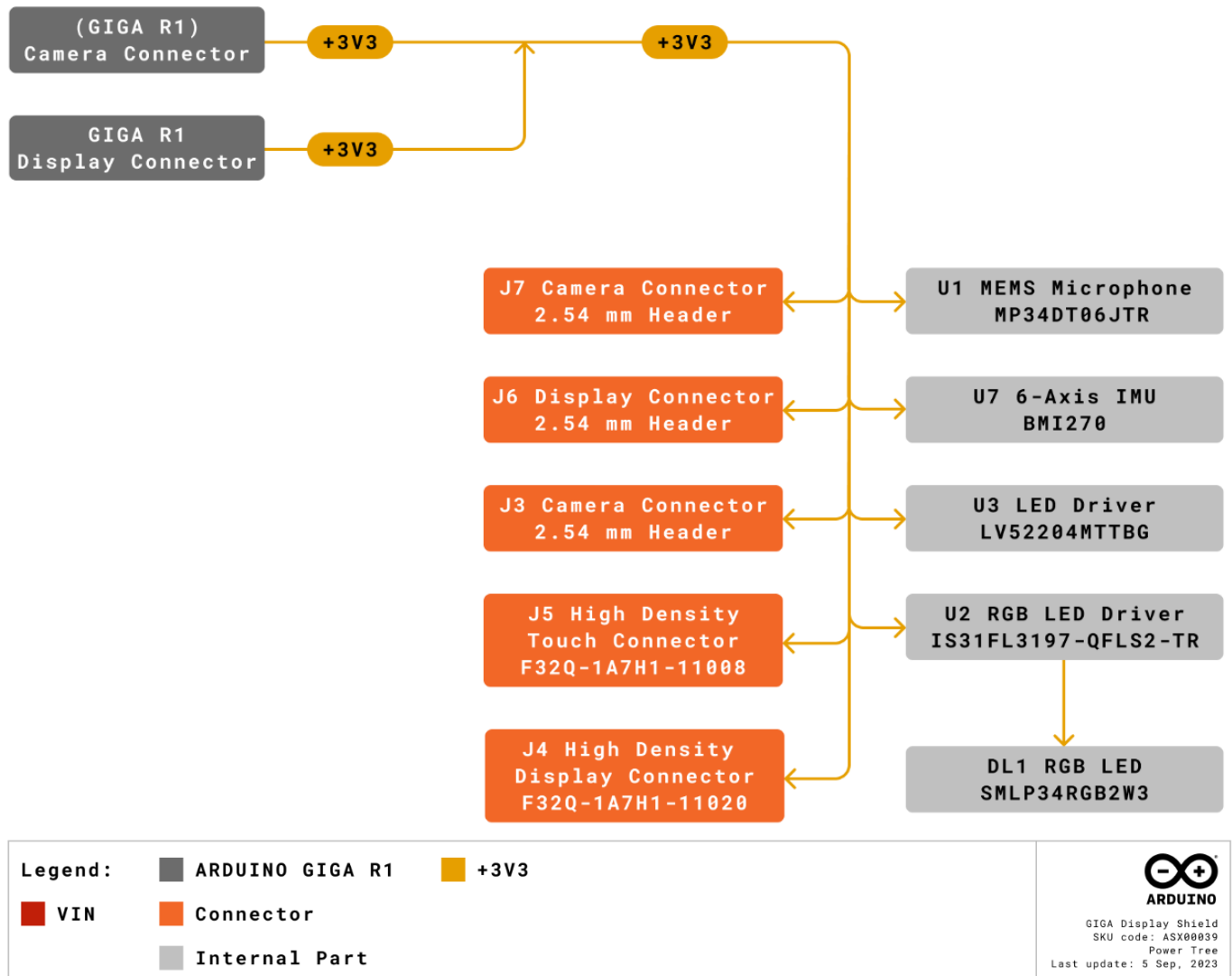
Arduino GIGA Display Shield Power Tree
