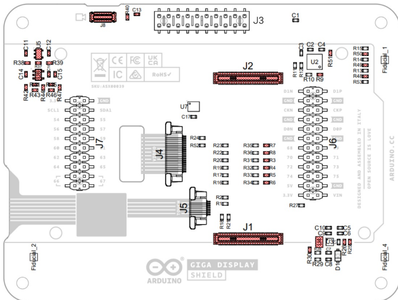
Back View of Arduino GIGA Display Shield
