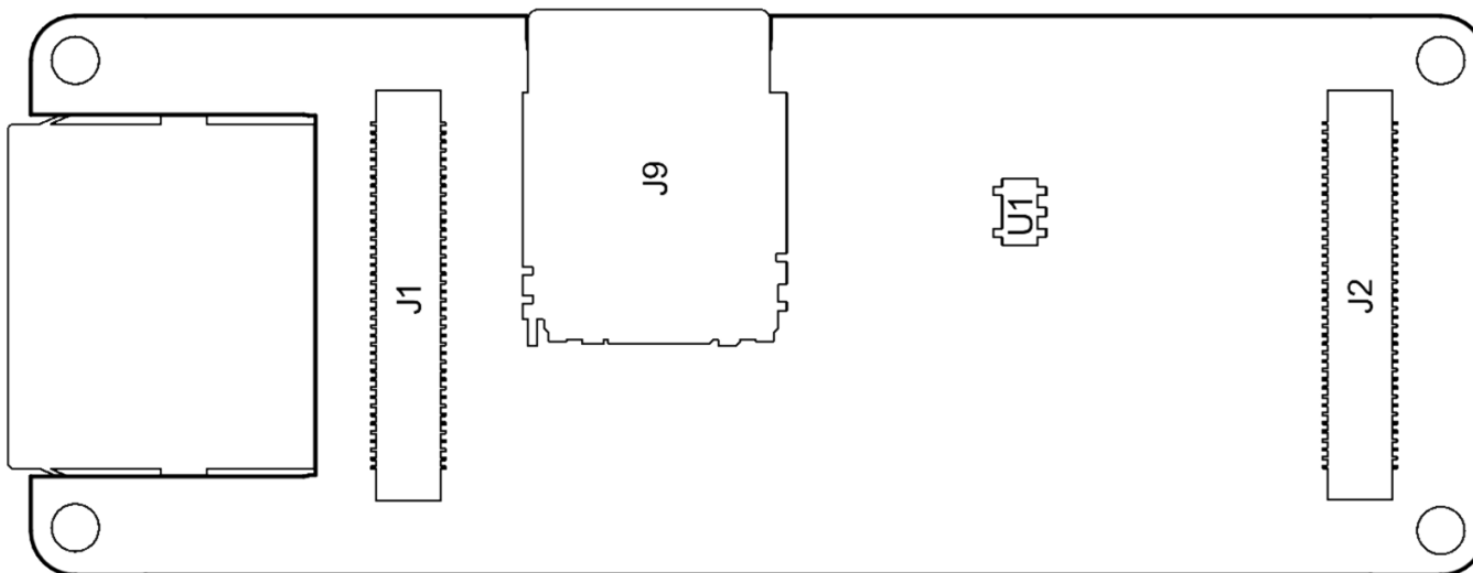
Bottom view
