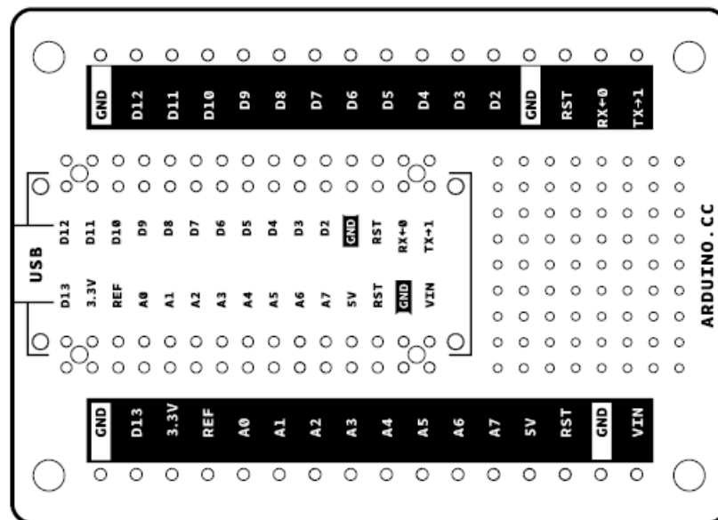
Board topology Top
