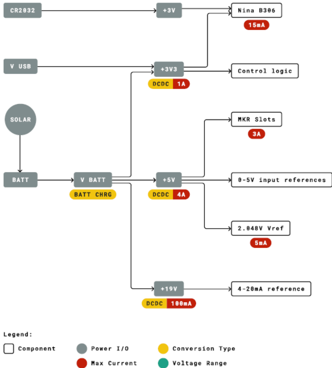
Edge Control Power Tree
