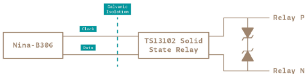
Solid state Relays schematic
