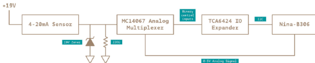
Low power sensors schematic
