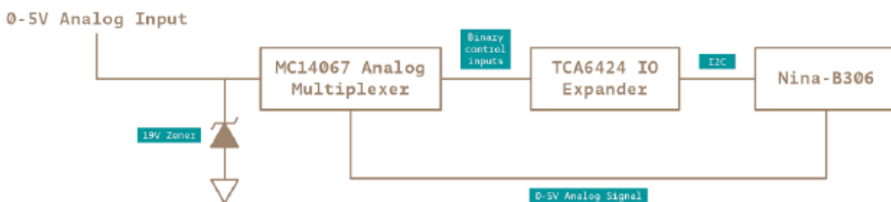
Analog Sensors schematic
