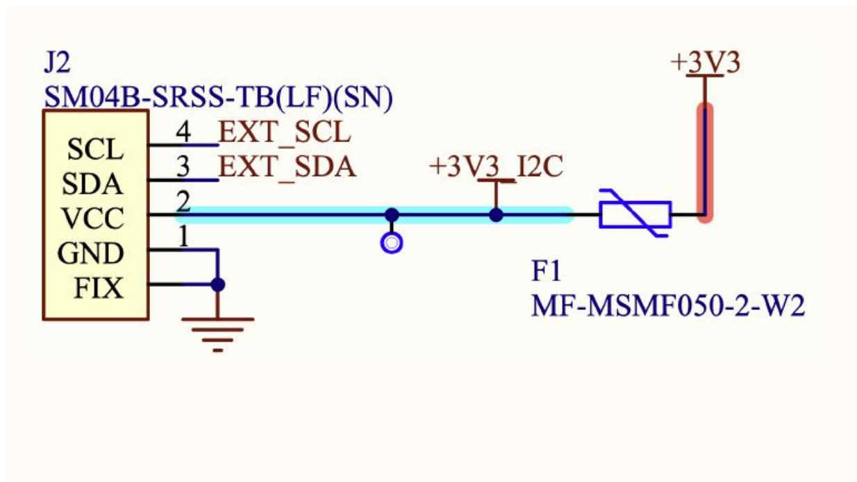
I2C connector.
