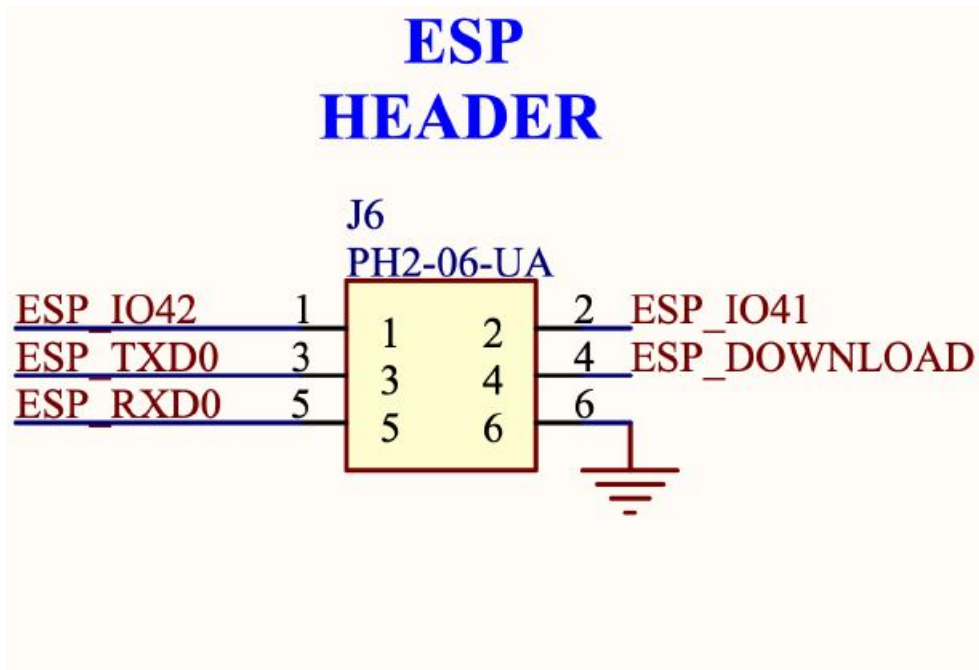
ESP header (schematic)
