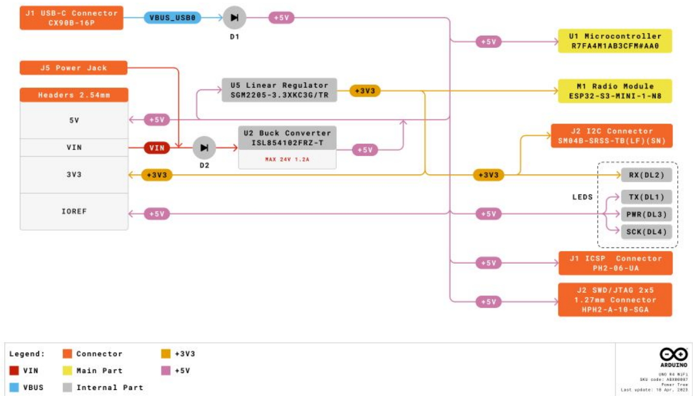
Arduino UNO R4 WiFi power tree.
