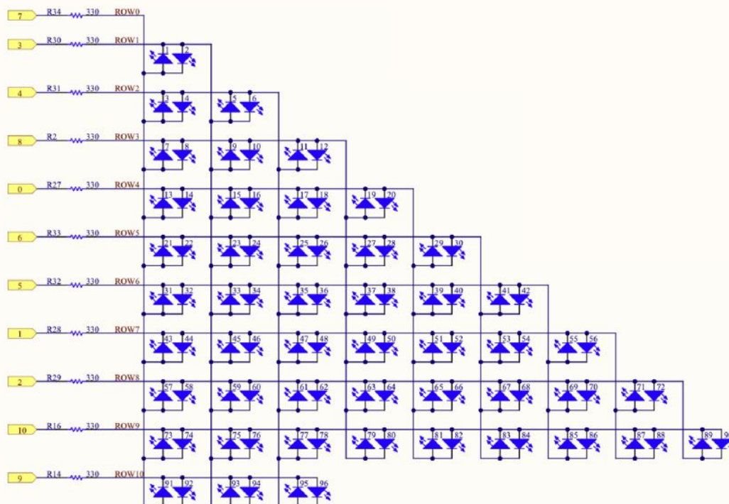
LED matrix schematics.
