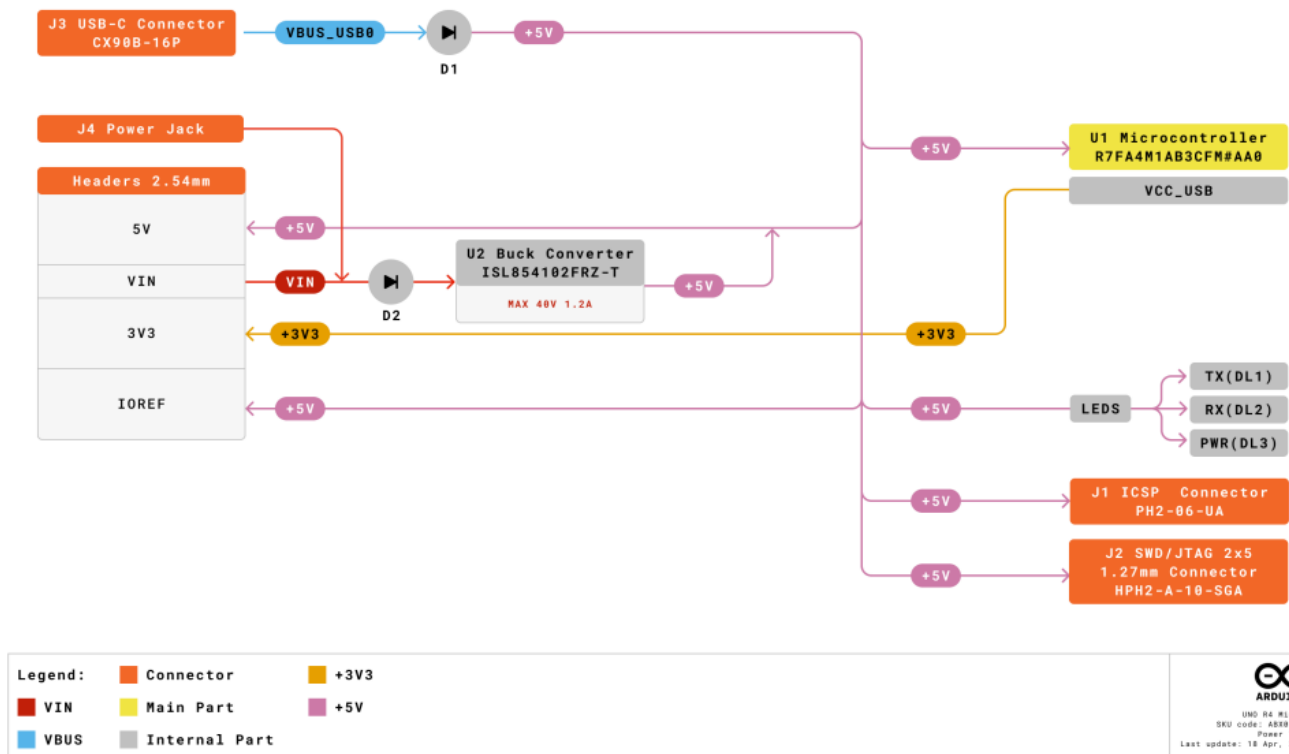
Arduino UNO R4 Minima power tree.
