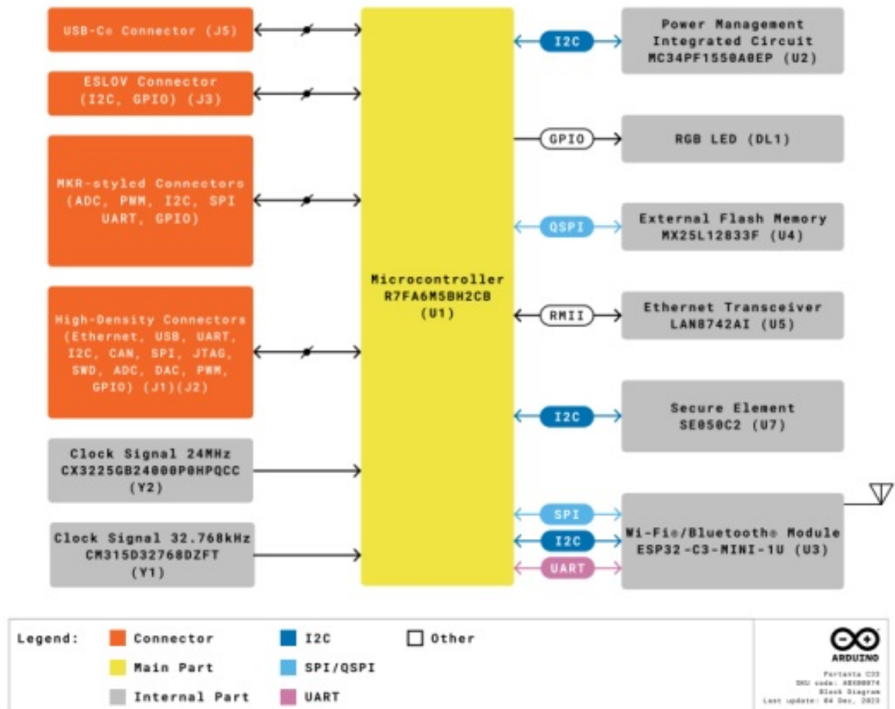
Figure 3. High-level architecture of the Portenta C33
