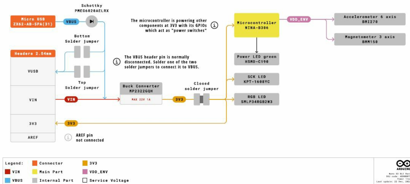
Power tree
