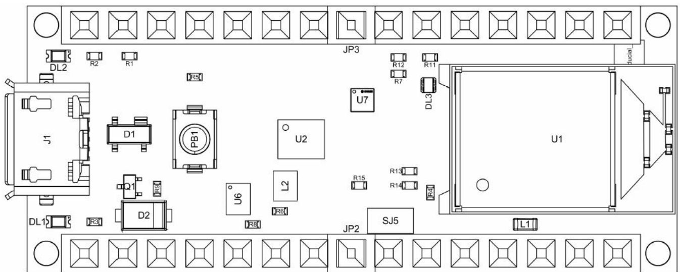
Board topology top
