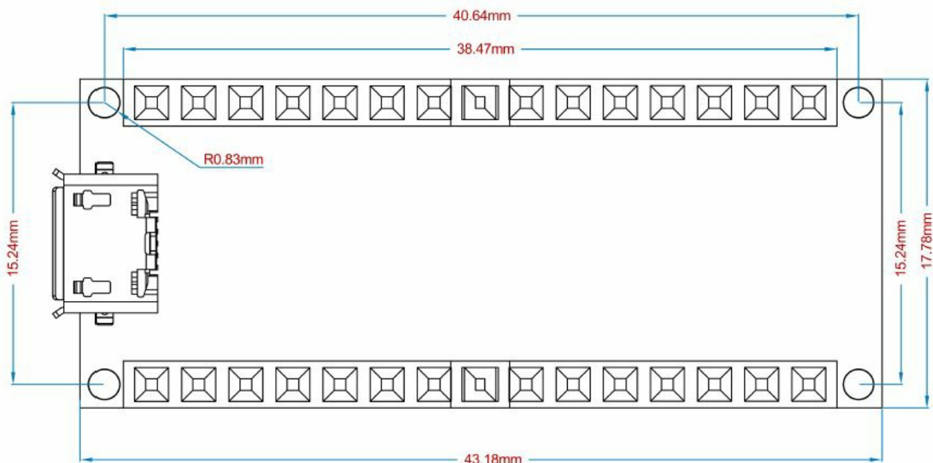
Board layout
