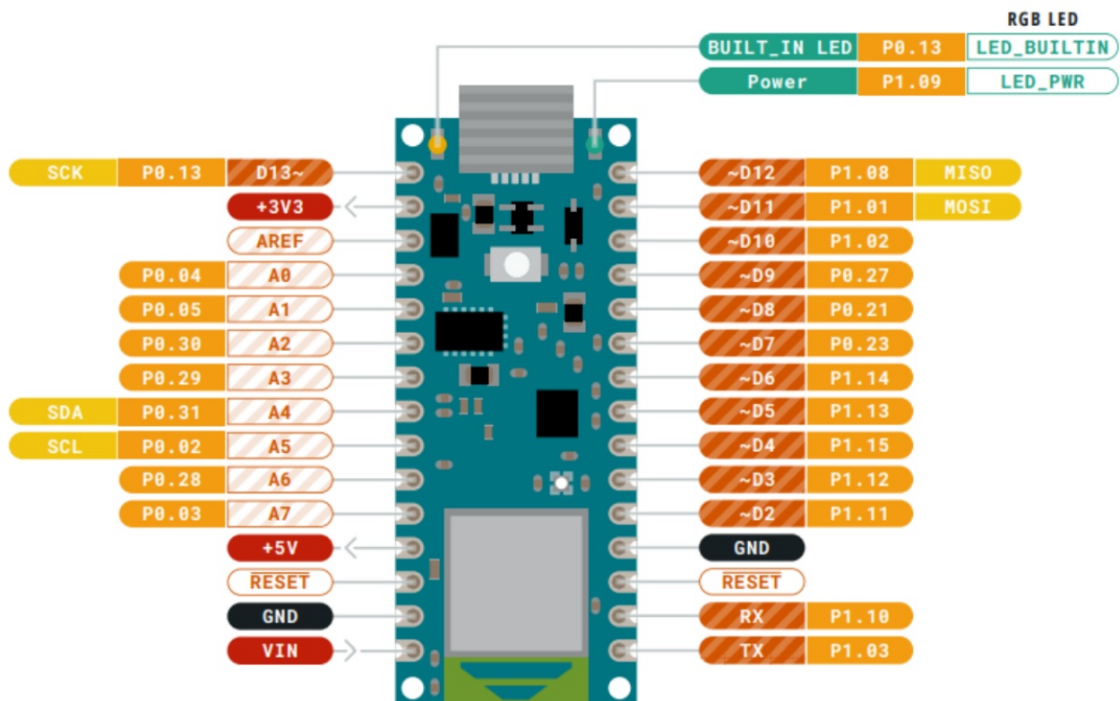
Pinout
