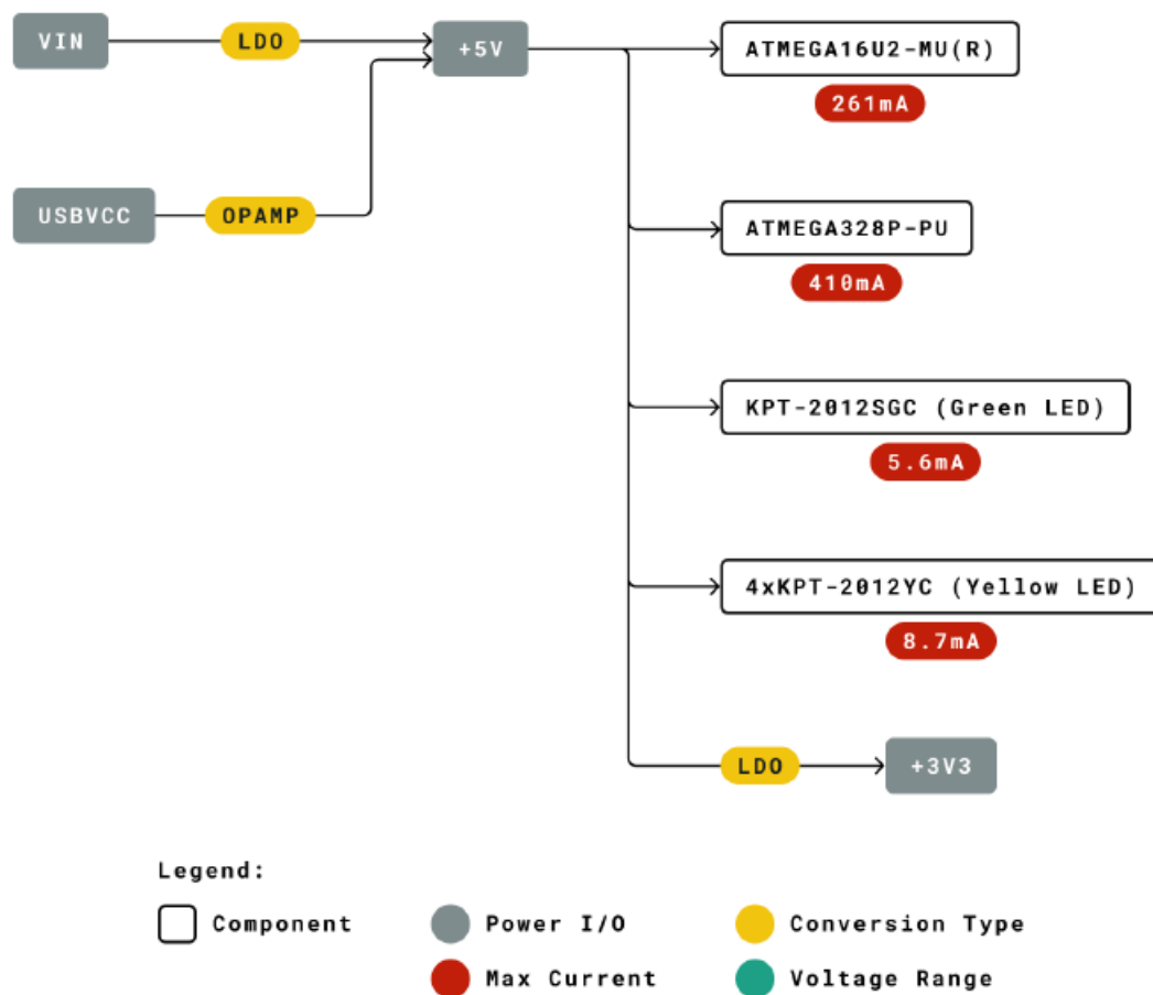
Power tree
