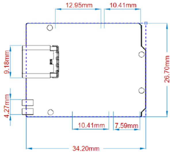
Board outline
