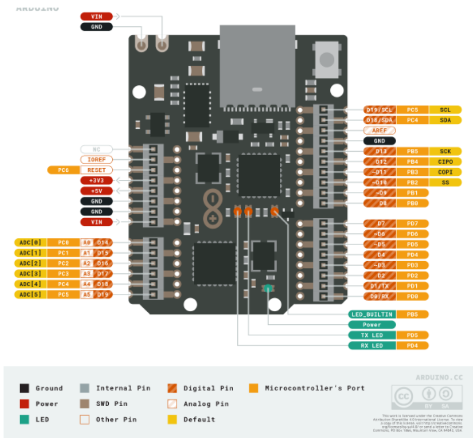
Pinout
