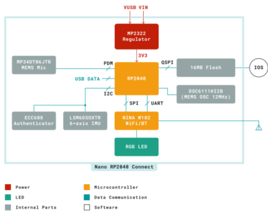
Block Diagram of Arduino Nano RP2040 Connect
