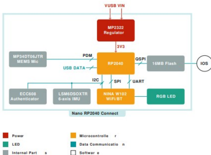
Block Diagram of Arduino Nano RP2040 Connect
