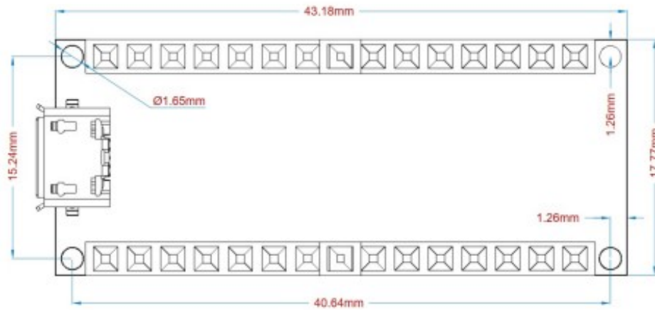
Back View of Arduino Nano RP2040 Connect Topology
