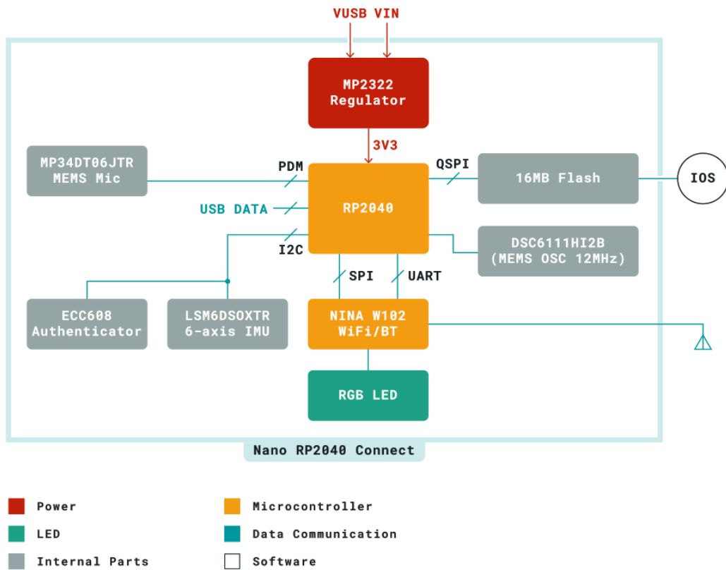
Block Diagram of Arduino Nano RP2040 Connect
