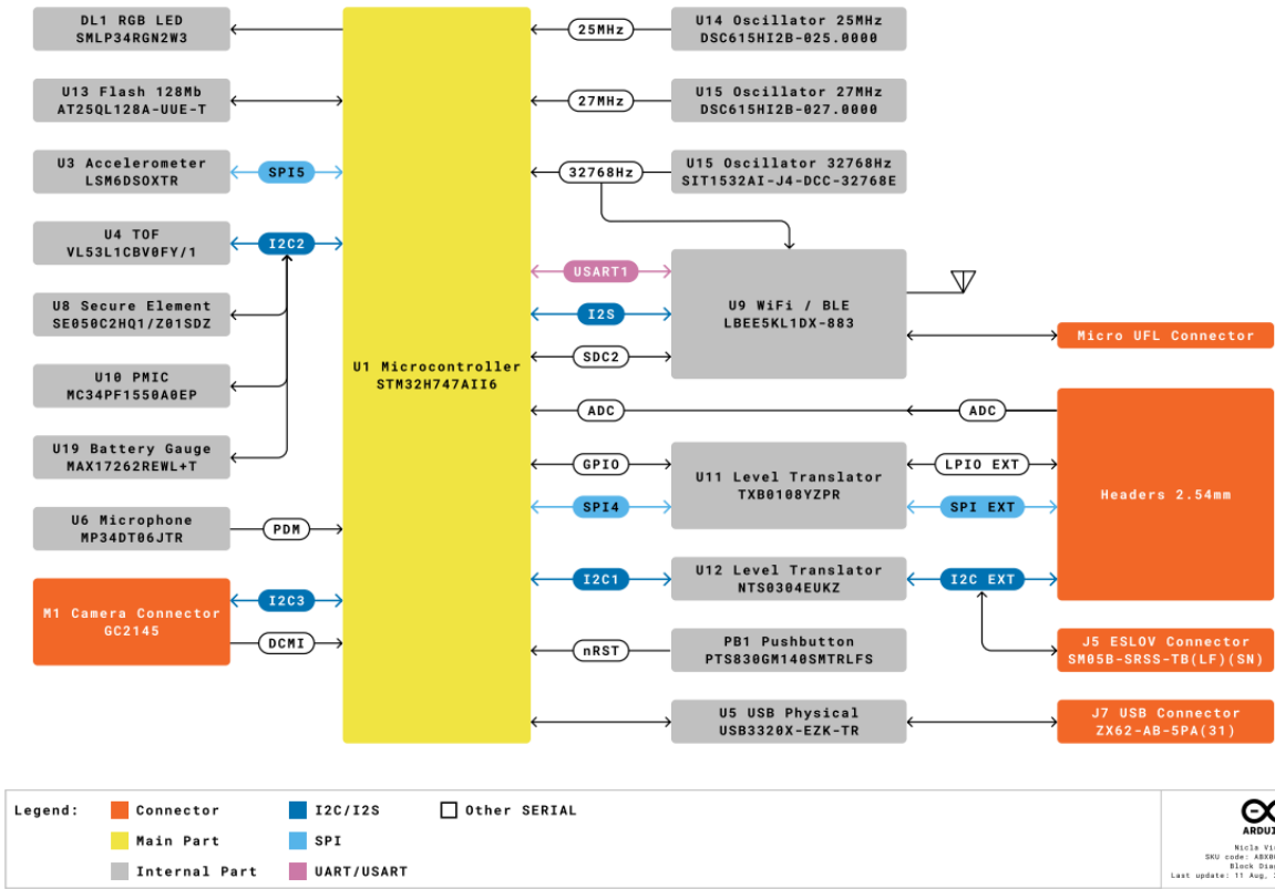
Nicla Vision Block Diagram
