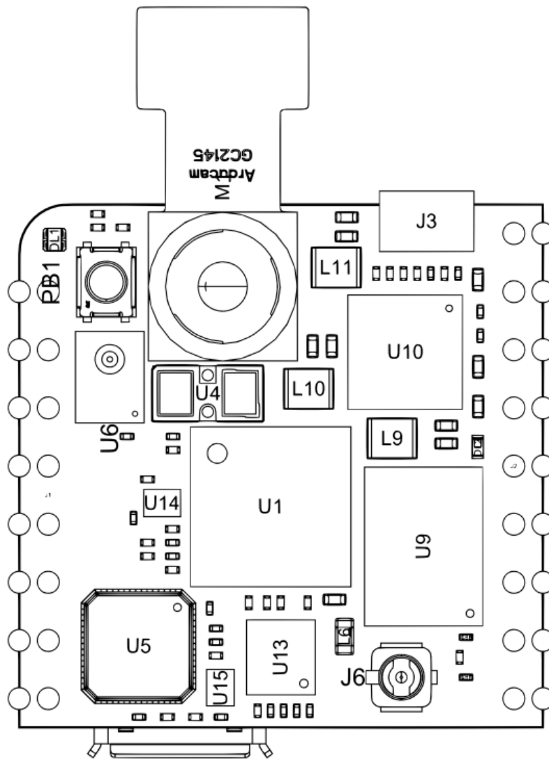
Nicla Vision Top View
