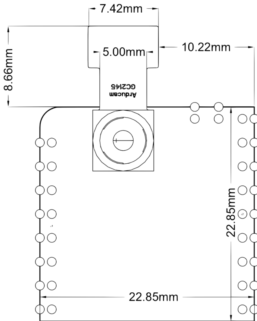
Nicla Vision Mechanical Drawing
