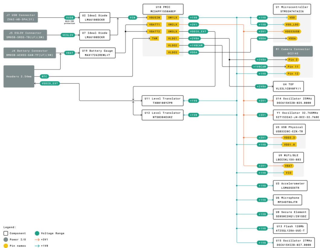
Nicla Vision Power Tree
