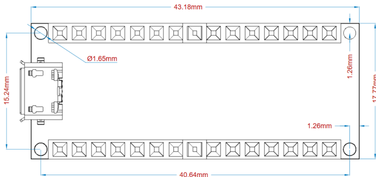
Mechanical dimensions of Arduino Nano RP2040 Connect
