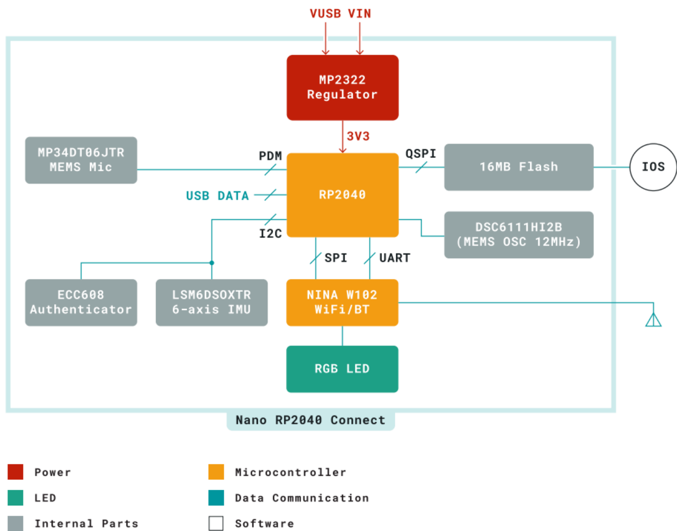
Block Diagram of Arduino Nano RP2040 Connect
