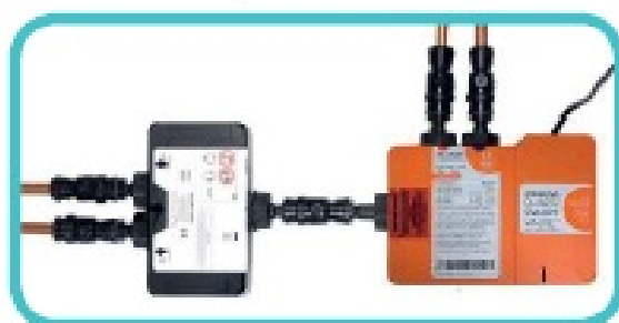
Quartz™ smart valve connected directly to diverter valve
