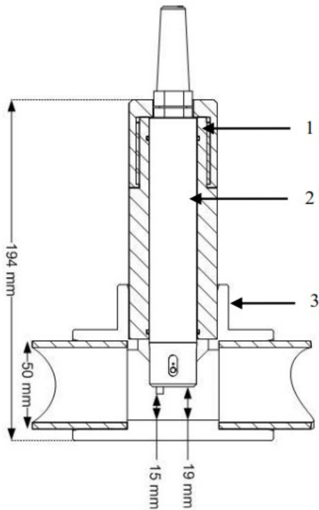
Mounting system for C4E sensor (PF-ACC-C-00226)
