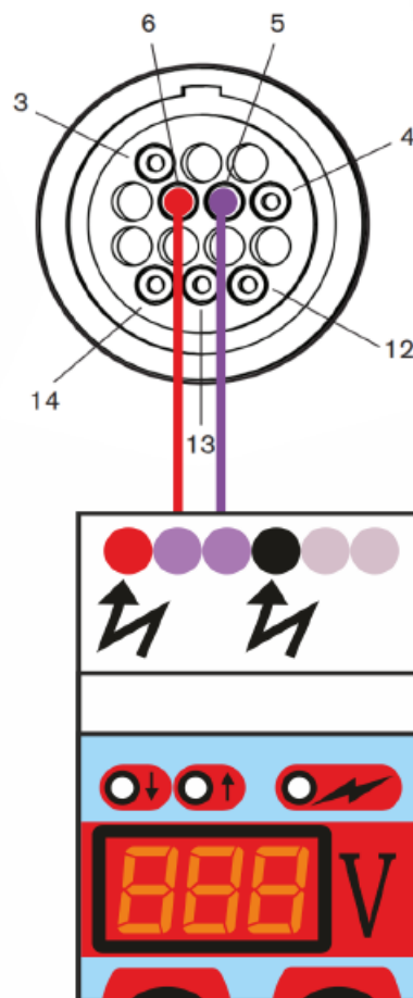
Hypertherm Powermax45 DV1:50 Connection
