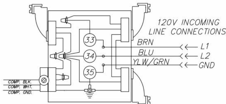
ELECTRICAL CONNECTIONS FOR MODEL 40HHC
