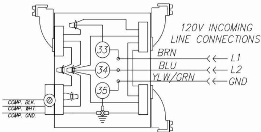
ELECTRICAL CONNECTIONS FOR MODEL 32HHC
