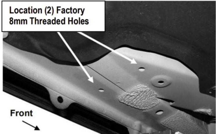
(Fig 1) Driver Side Front Mounting Location
