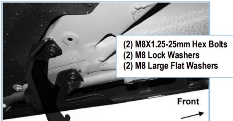
( Fig 2 ) Driver Front Mounting Bracket (DFM) Installation
