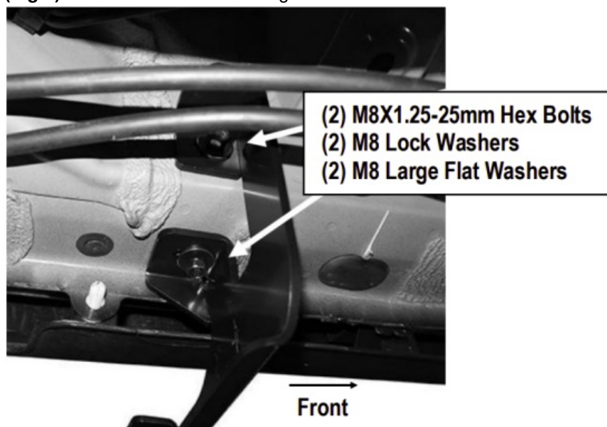
(Fig 6) Driver Rear Mounting Bracket Installation
