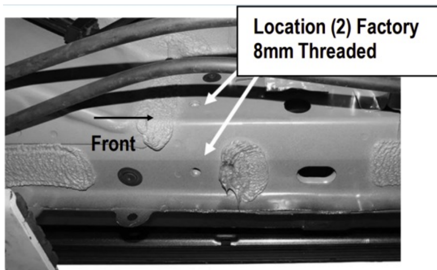
(Fig 5) Driver Side Rear Mounting Location
