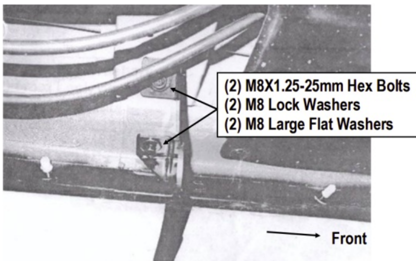
( Fig 4 ) Driver Center Mounting Bracket Installation
