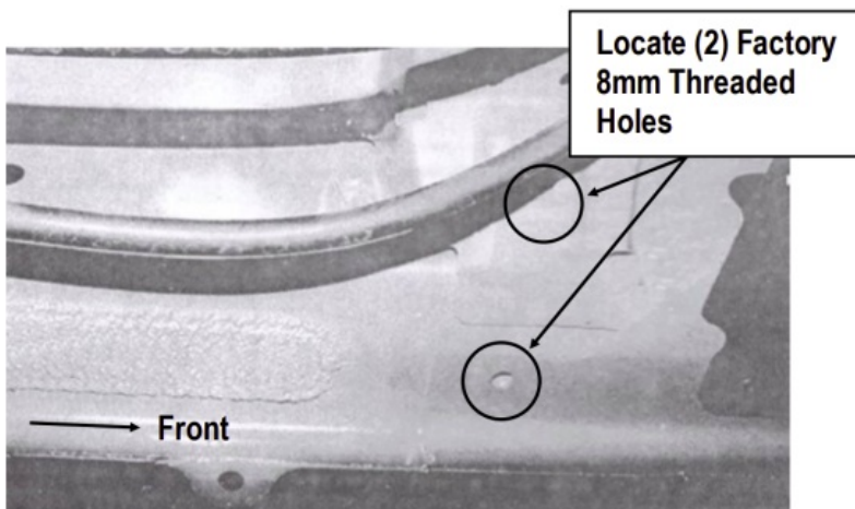
( Fig 3 ) Driver Side Center Mounting Location
