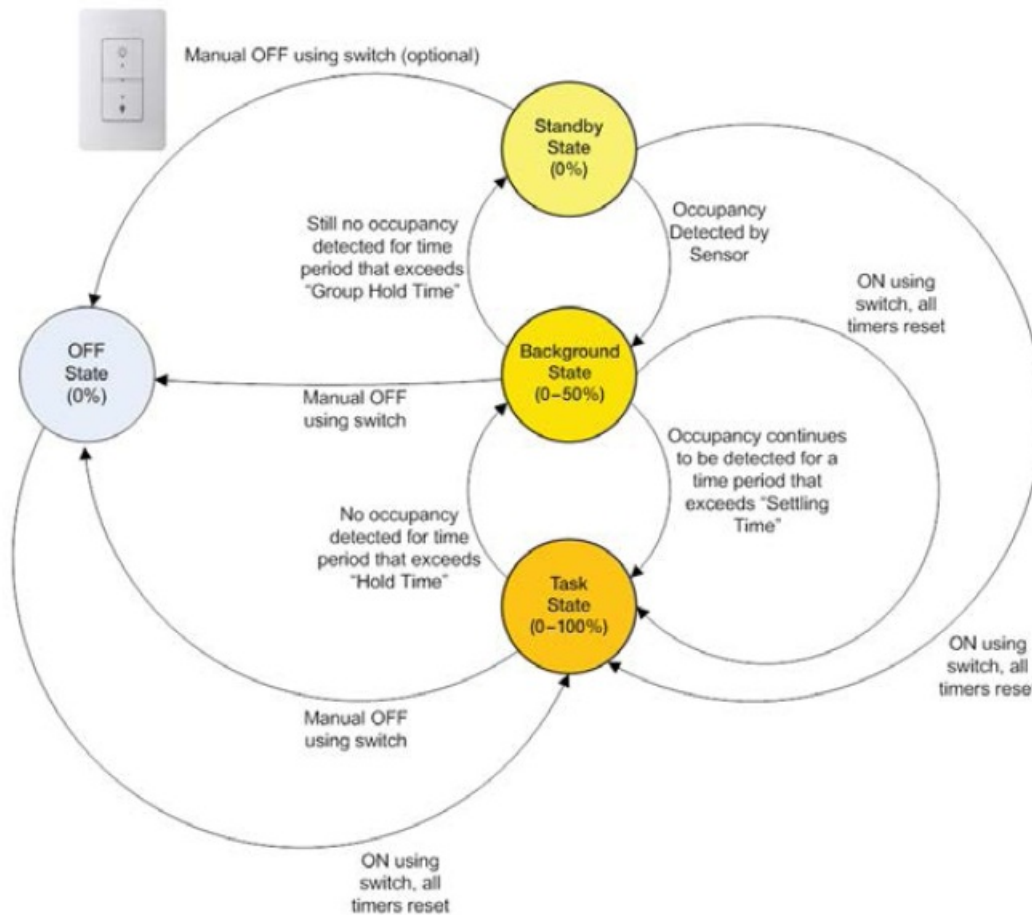
Figure 2: (EXAMPLE) State Changes in Automatic Mode after commissioning
