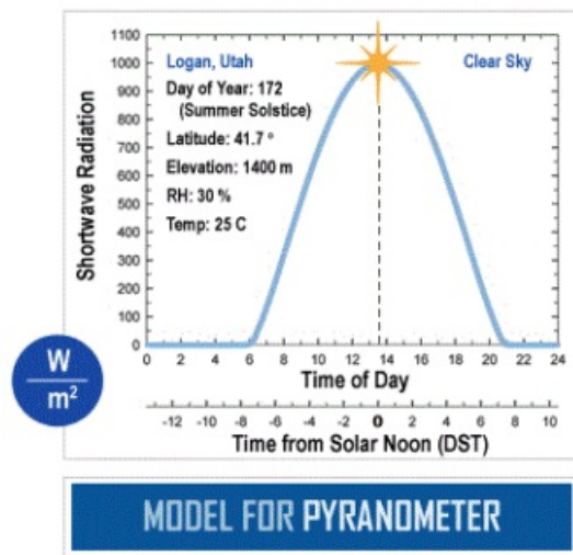
SHORTWAVE RADIATION
