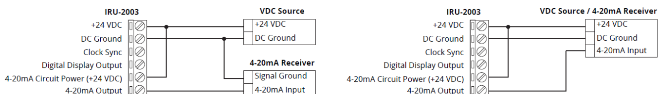
Figure 1.2 - Single VDC Source Wiring
