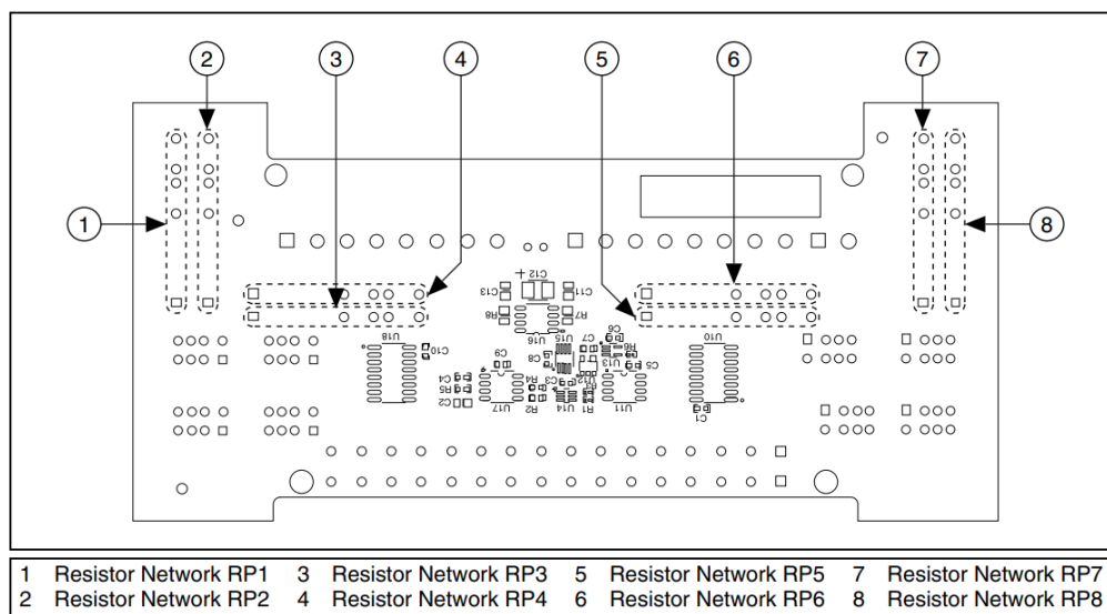
Figure 3. Resistor Network Locator Diagram
