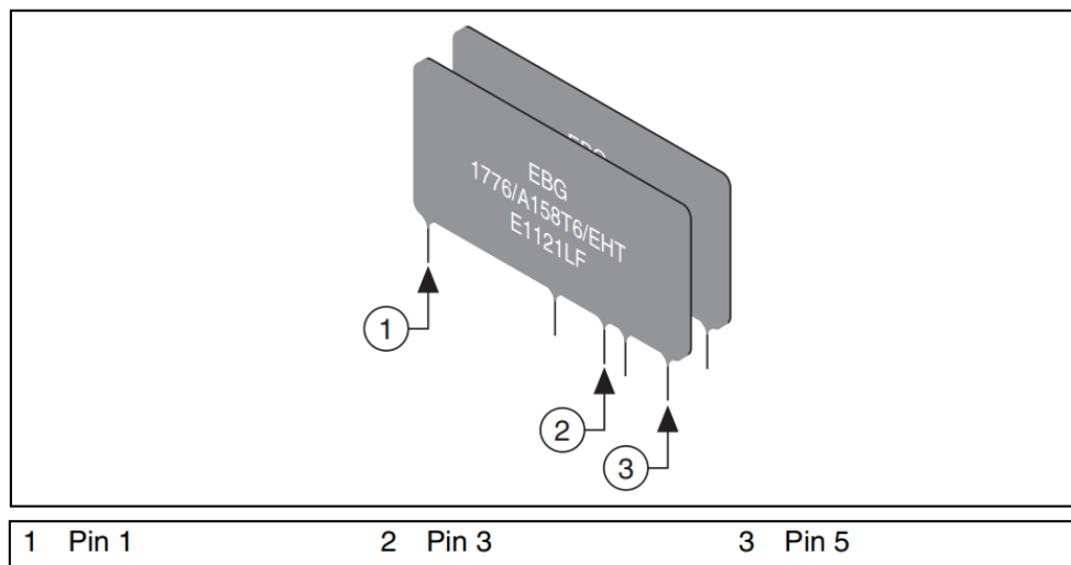
Figure 1. SCXI-1313A Resistor Network Pin Designations
