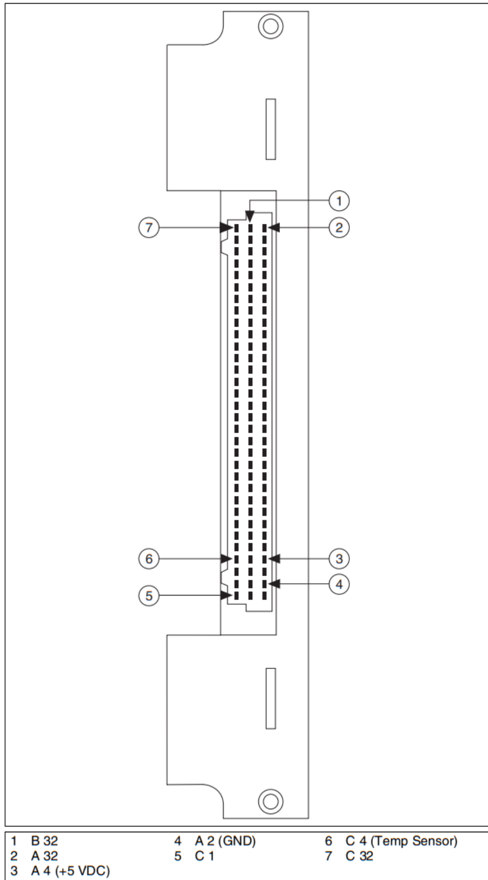
Figure 4. SCXI-1313A Connector Pin Assignments
