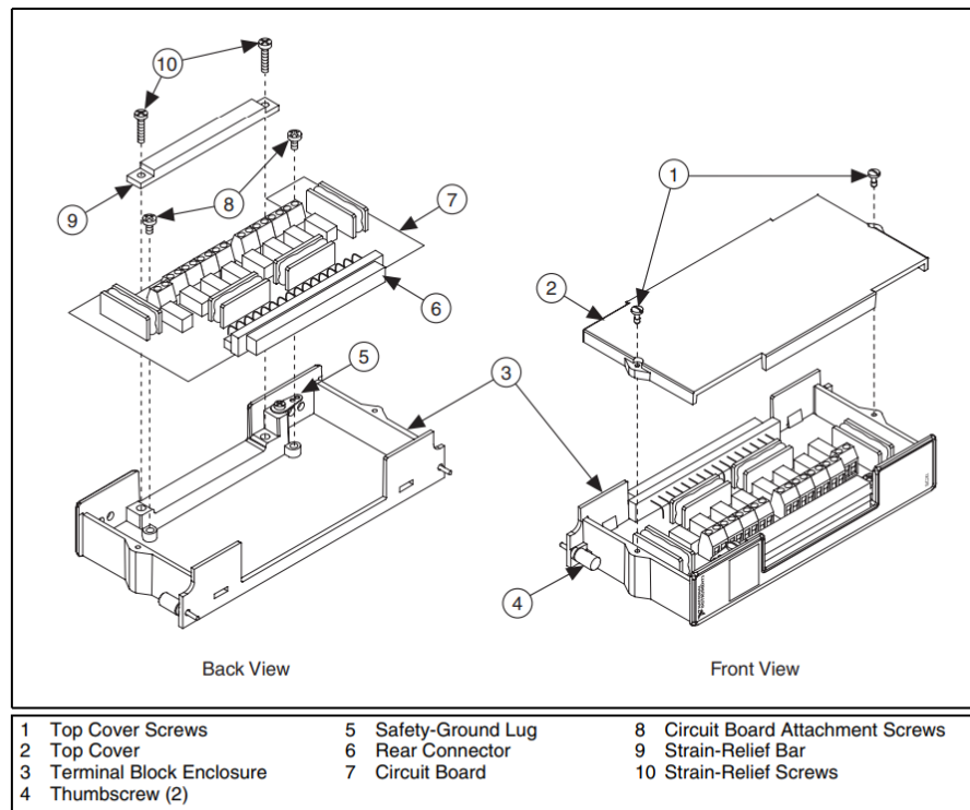
Figure 2. SCXI-1313A Parts Locator Diagram
