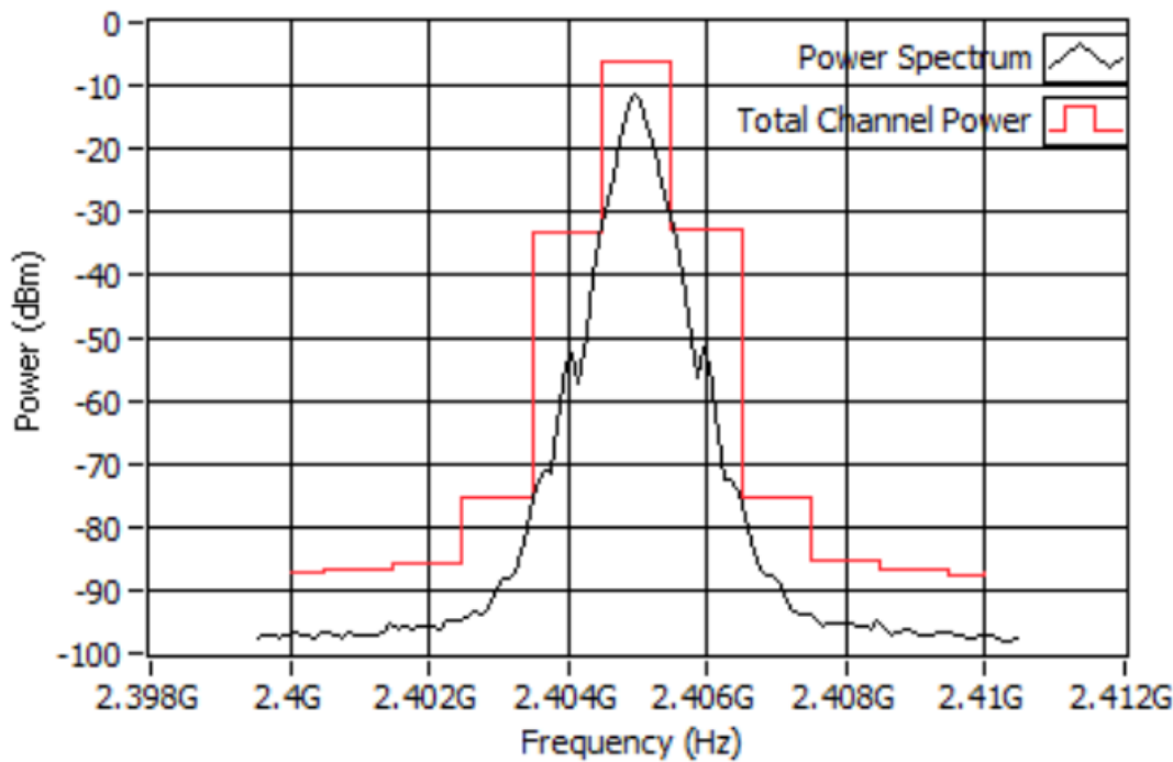
Figure 3. Tx output power spectrum measurement
