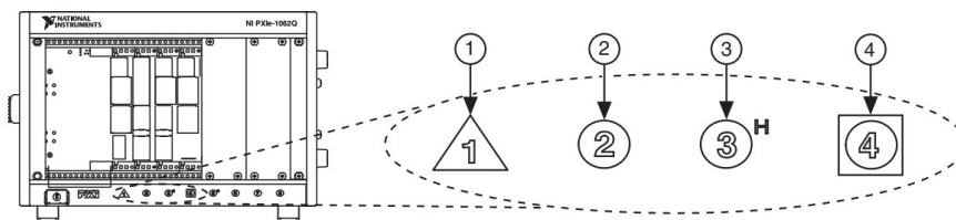
Figure 4. Symbols for PXI Express/PXI Express Hybrid/PXI Slots
