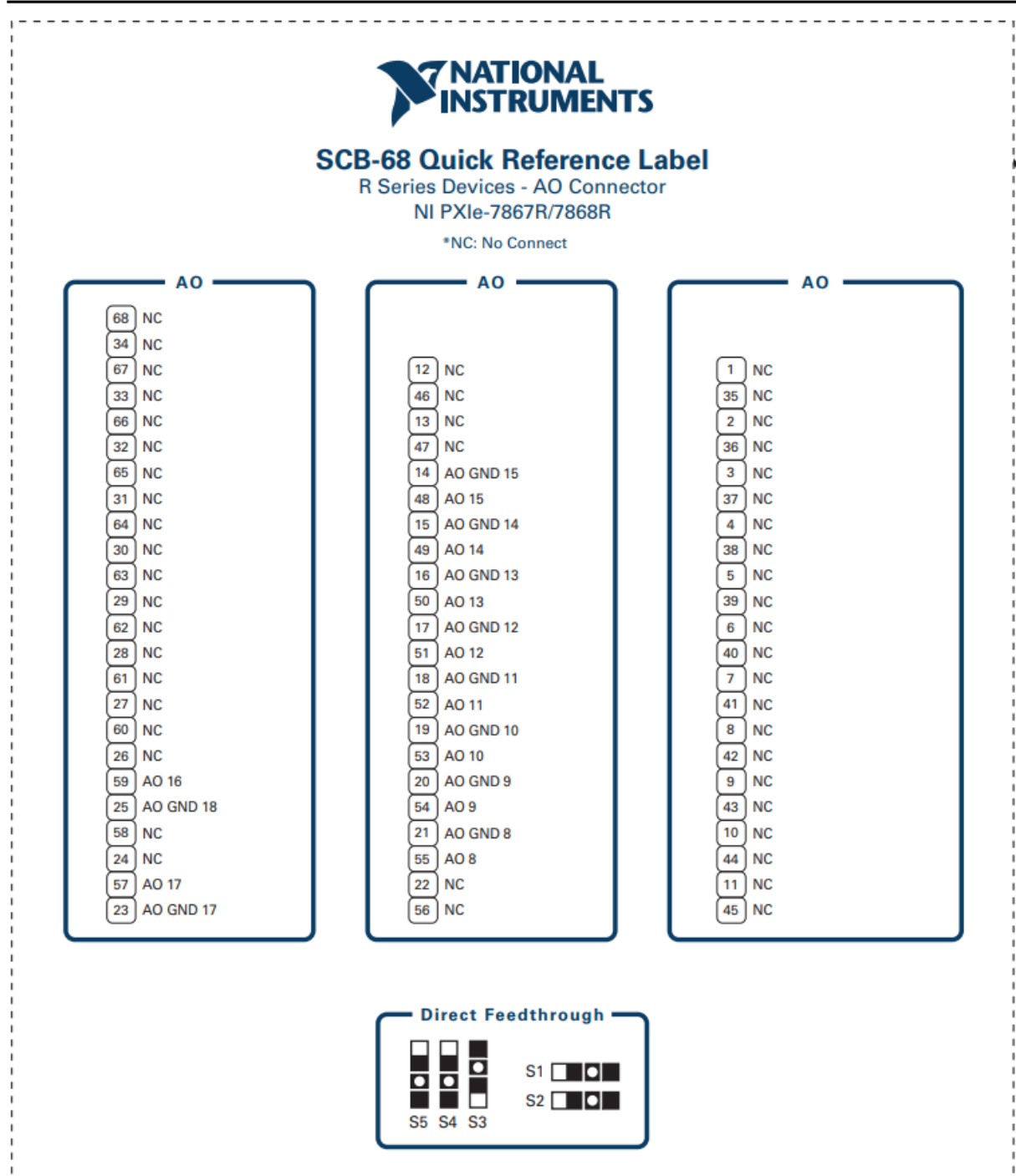
Figure 2. RAO Connector for NI PXIe-7867R/7868R
