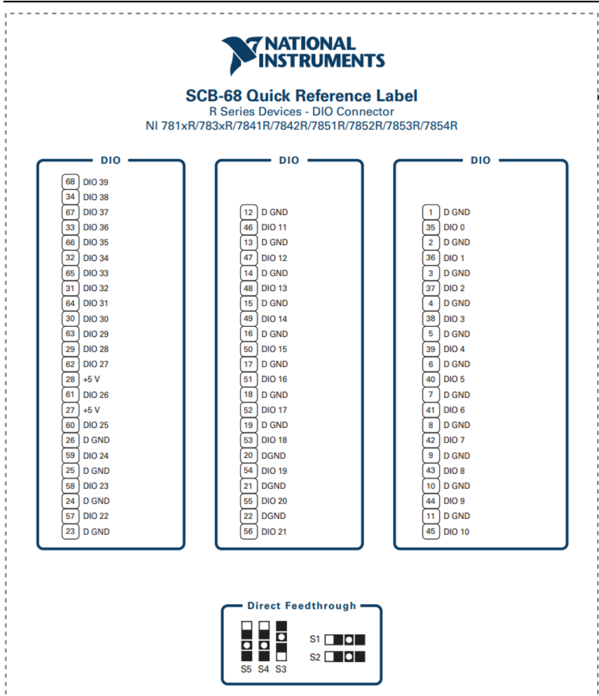
Figure 1. RMIO Connector for NI PXIe-7867R/7868R
