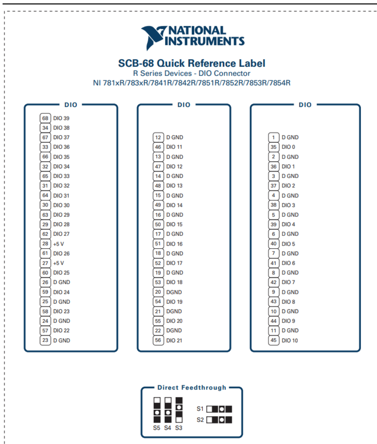
Figure 4. RDIO Connector for NI 781xR/783xR/7841R/7842R/7851R/7852R/7853R/7854R
