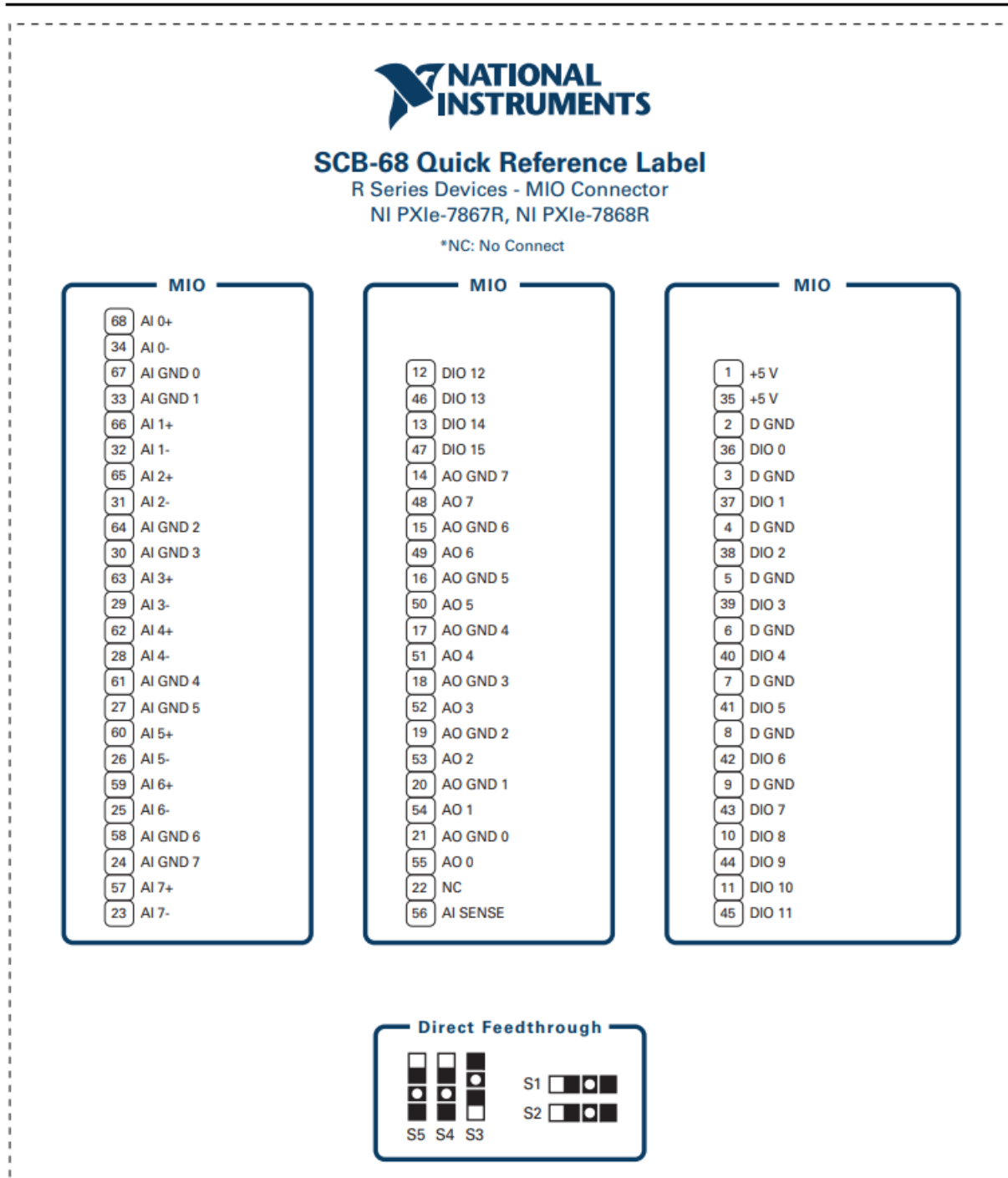
Figure 3. RMIO Connector for NI 781xR/783xR/784xR/785xR
