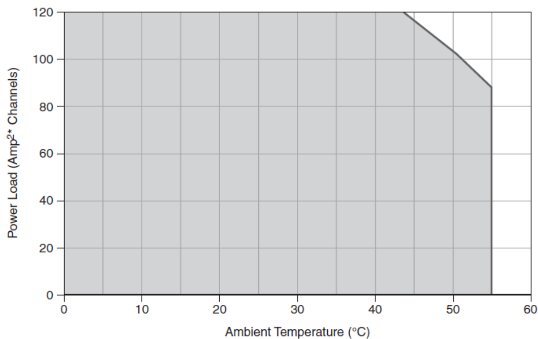
Figure 1. Module Load Derating
