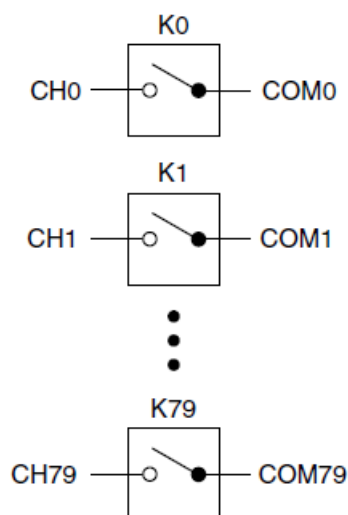
Figure 2. NI PXI-2520 Hardware Diagram
