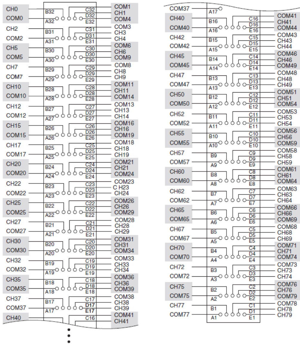
Figure 3. NI PXI-2520 Connector Pinout
