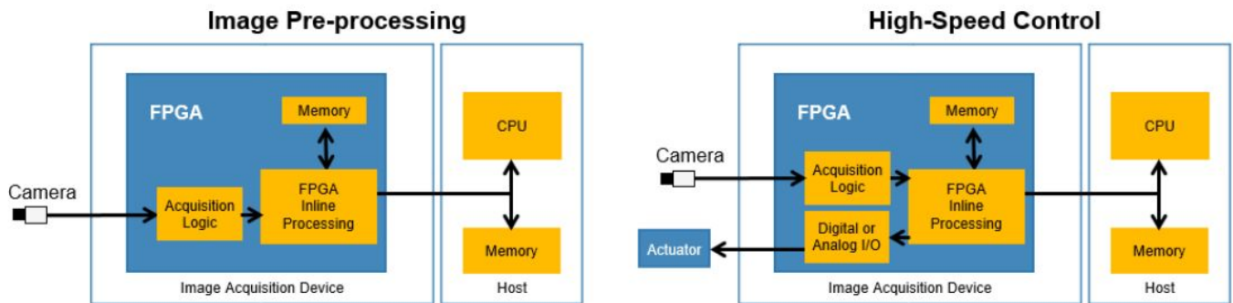
Figure 1. Use cases for inline FPGA image processing
