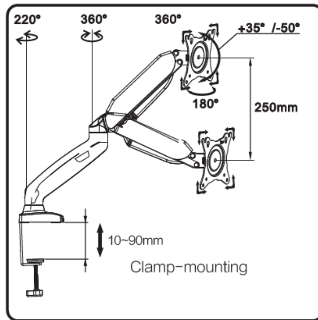
Diagram of fully-assembled monitor arm spec in depth
