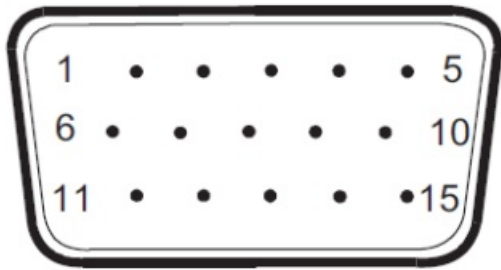
15-Pin Color Display Signal Cable
