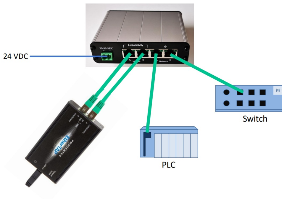
Figure 2 - Connecting the EtherTAP to the EtherMIRROR
