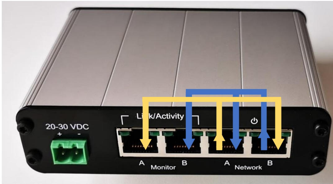
Figure 1 - Internal connections
