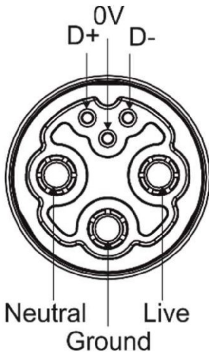
Output – panel connector (front view)
