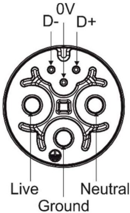
Output – panel connector (front view)
