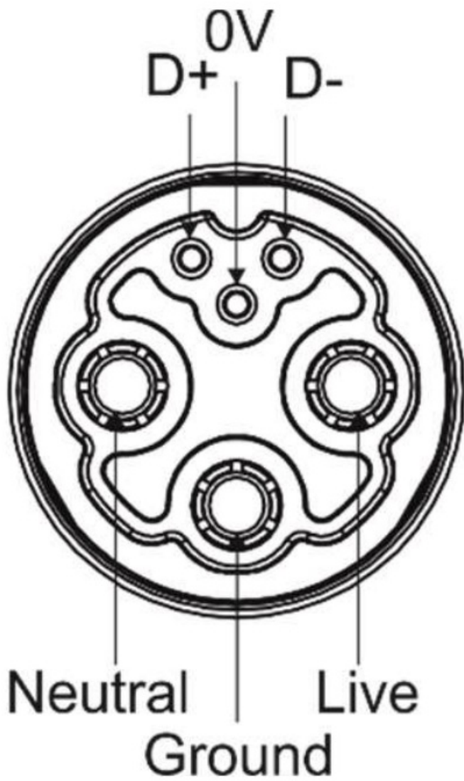
Output – panel connector (front view)
