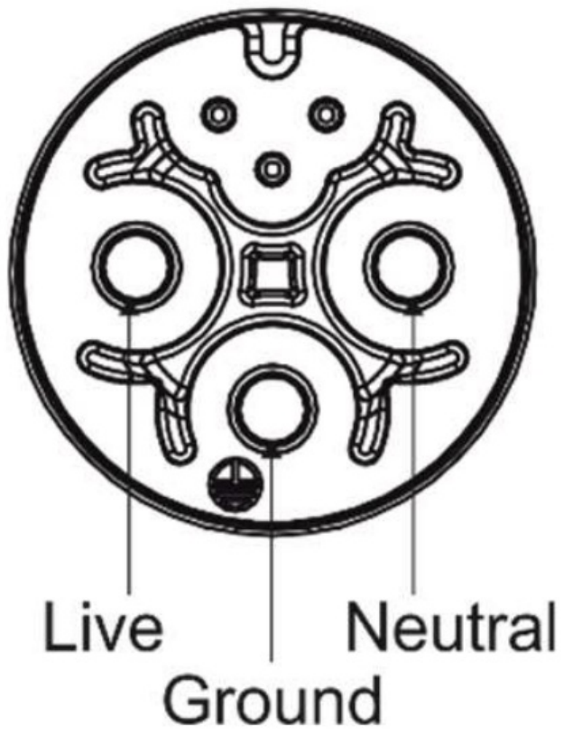
Output – panel connector (front view)
