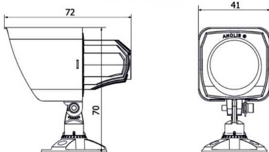
Fixture with top hat
