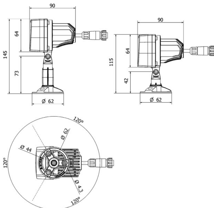
Fixture with half top hat
