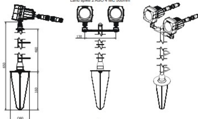
Land spike 2 ASO 4 MC 500mm
