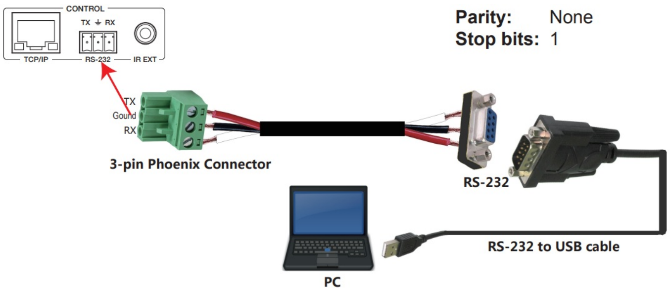
Figure 1: 3-pin phoenix connector to USB
