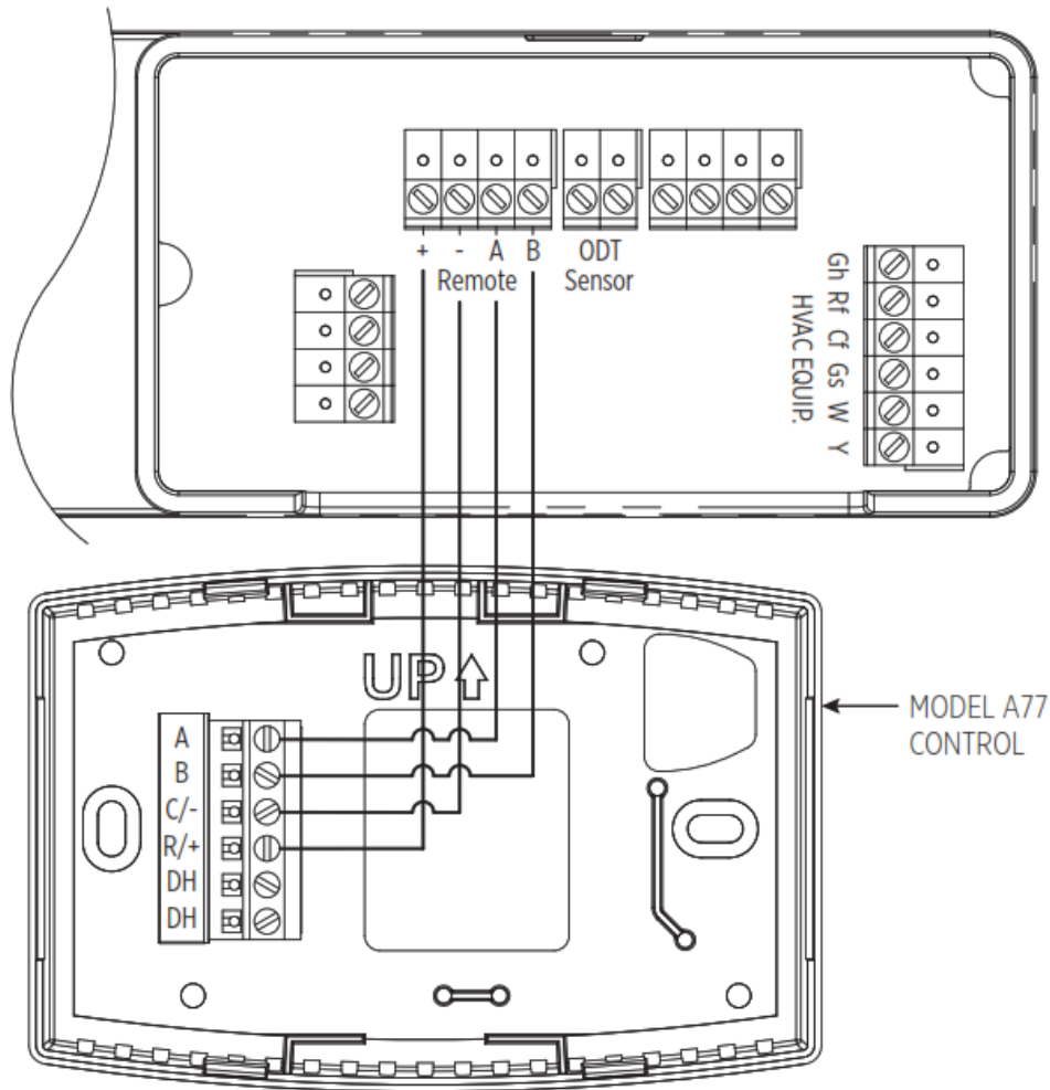
FIGURE 5 – MODEL A77 WIRING WITH ANDEN® DEHUMIDIFIERS
