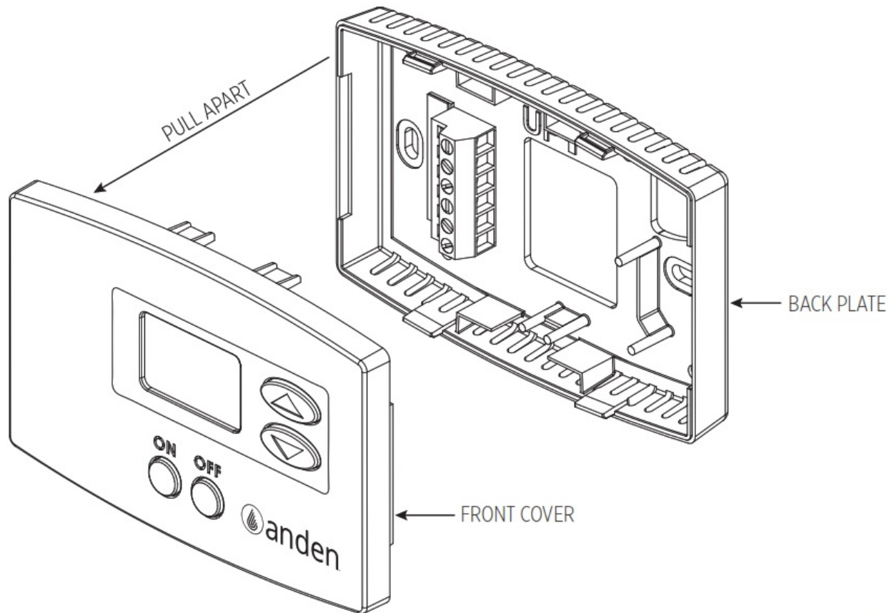
FIGURE 2 – DISASSEMBLE CONTROL
