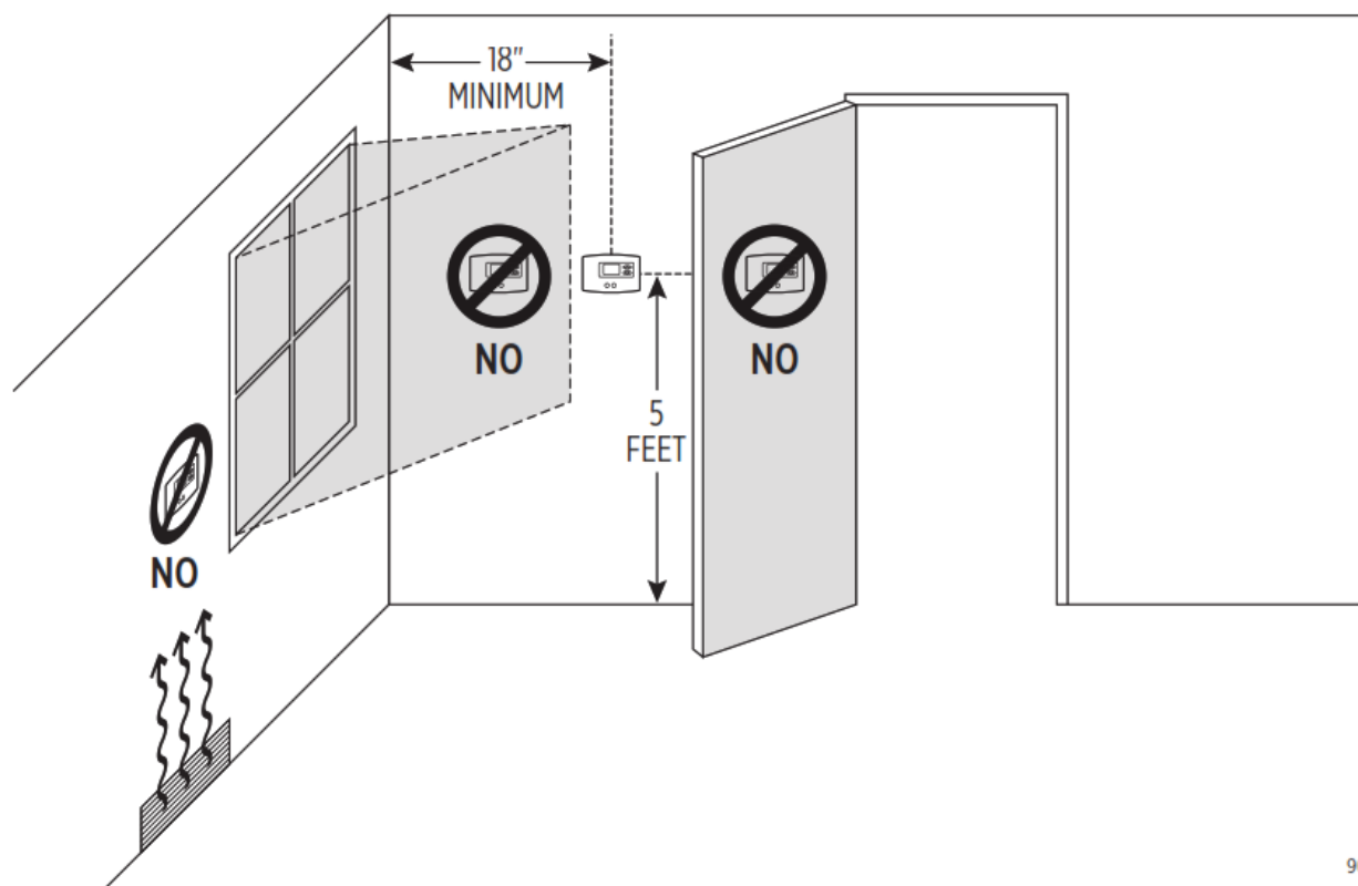
FIGURE 1 – MOUNTING LOCATION
