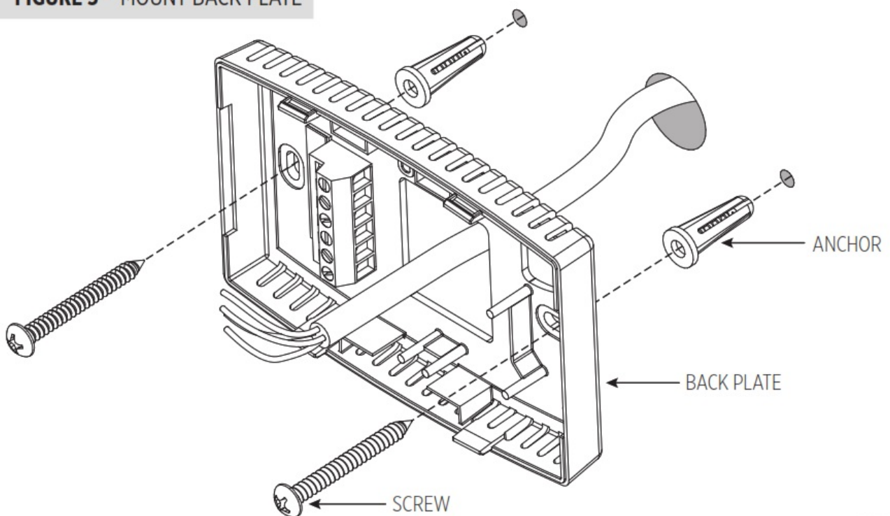
FIGURE 3 – MOUNT BACK PLATE
