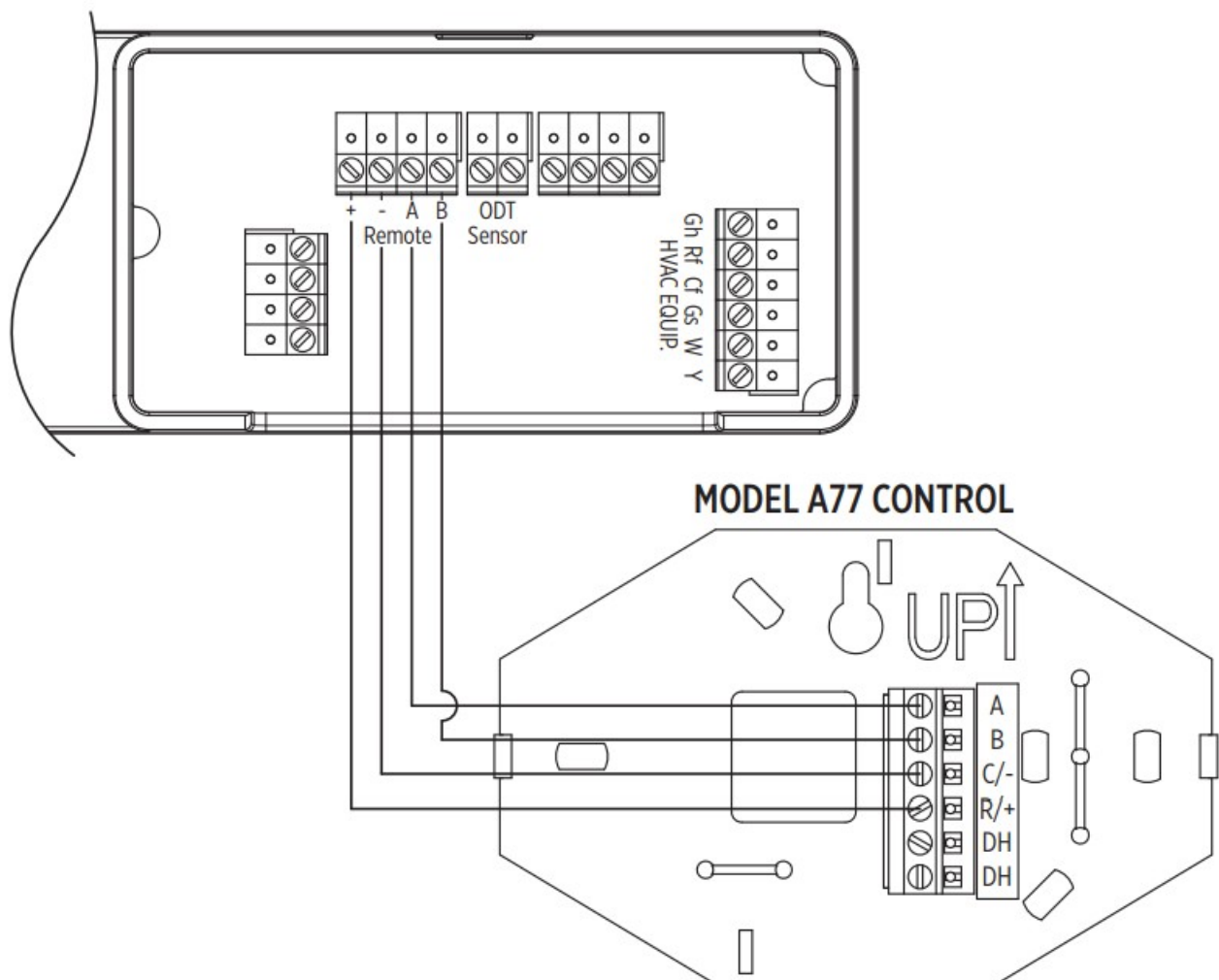
FIGURE 5 – MODEL A77 REMOTE CONTROL WIRING
