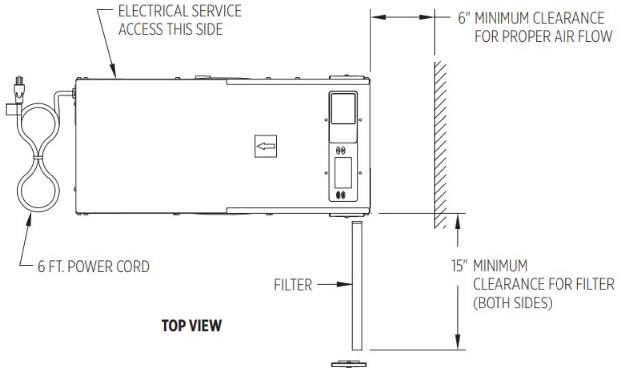
FIGURE 2 – FILTER ACCESS CLEARANCE
