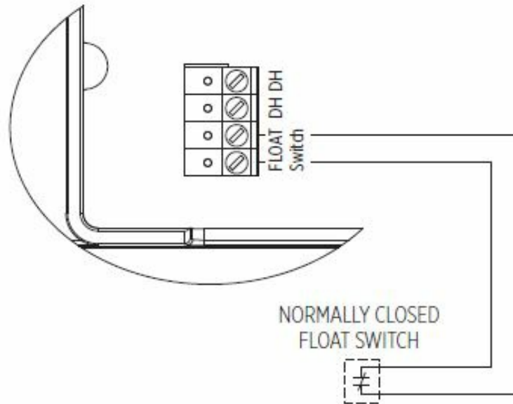
FIGURE 9 – FLOAT SWITCH WIRING
