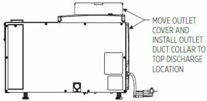
FIGURE 4 – FLOOR MOUNT INSTALL
