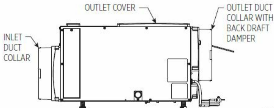
FIGURE 3 – HANGING INSTALL WITH DUCTING
