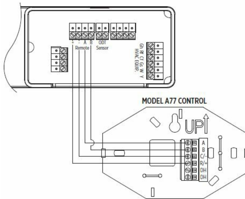
FIGURE 10 – MODEL A77 REMOTE CONTROL WIRING
