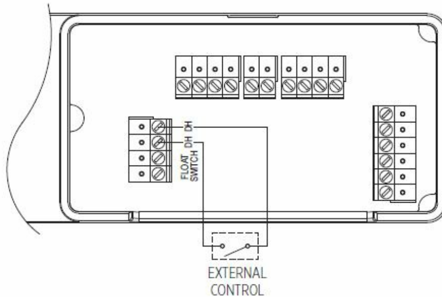
FIGURE 11 – ALTERNATE EXTERNAL CONTROL WIRING
