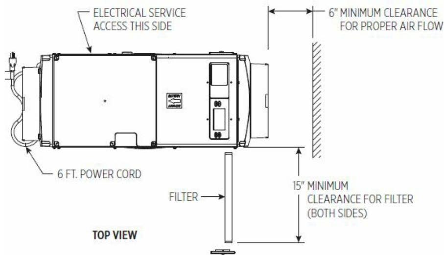
FIGURE 6 – FILTER ACCESS CLEARANCE
