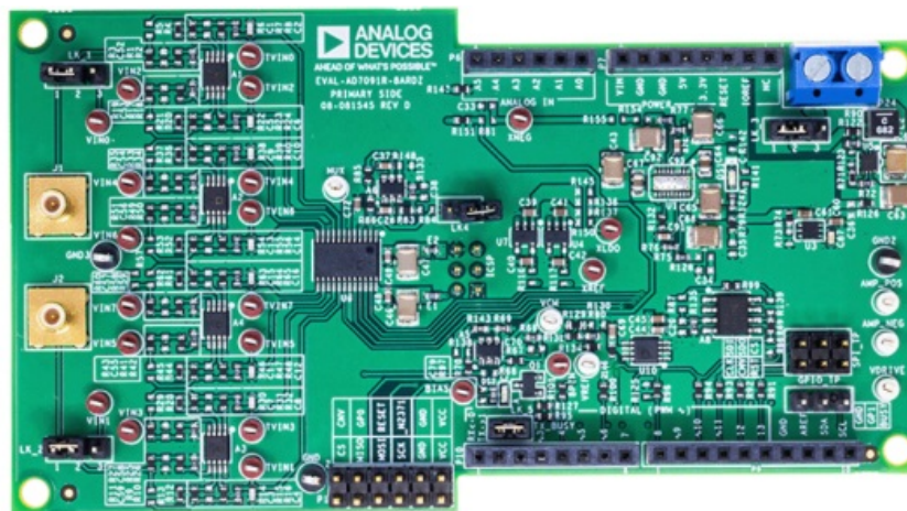
Figure 1. Evaluation Board Photograph
