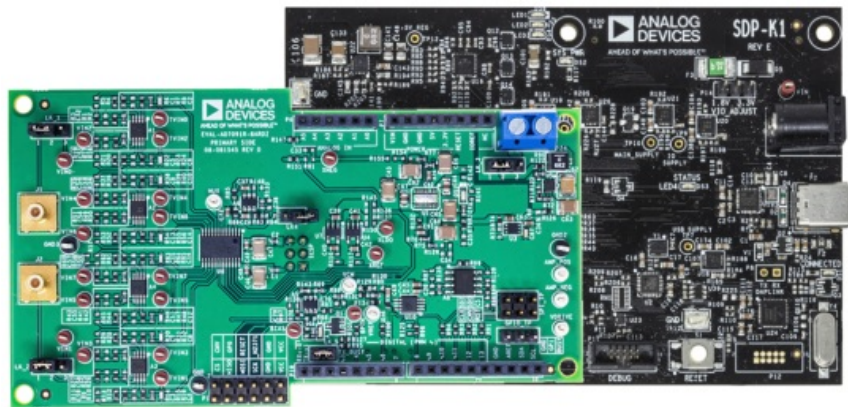
Figure 2. EVAL-AD7091R-8ARDZ (Left) Connected to the EVAL-SDP-CK1Z Board (Right)
