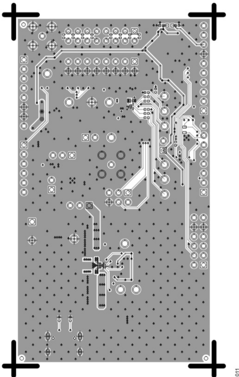
Figure 10. EVAL-AD3530RARDZ Bottom Side Routing
