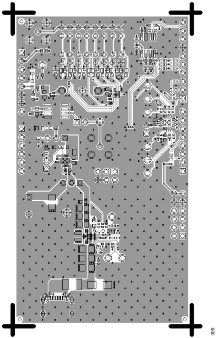
Figure 8. EVAL-AD3530RARDZ Top Side Routing
