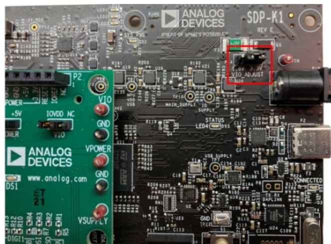
Figure 3. VIO_ADJUST Jumper on SDP-K1 Board
