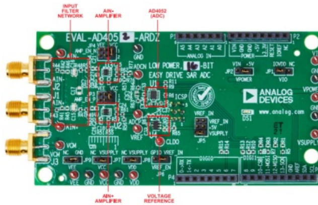
Figure 8. EVAL-AD4052-ARDZ Evaluation Board Circuitry Locations Top Side
