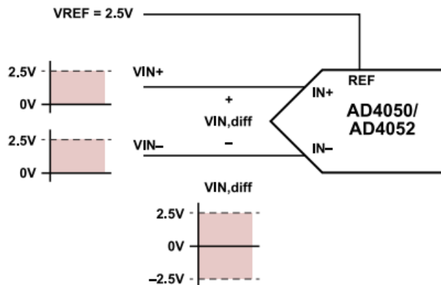
Figure 13. AD4050/AD4052 Input Range
