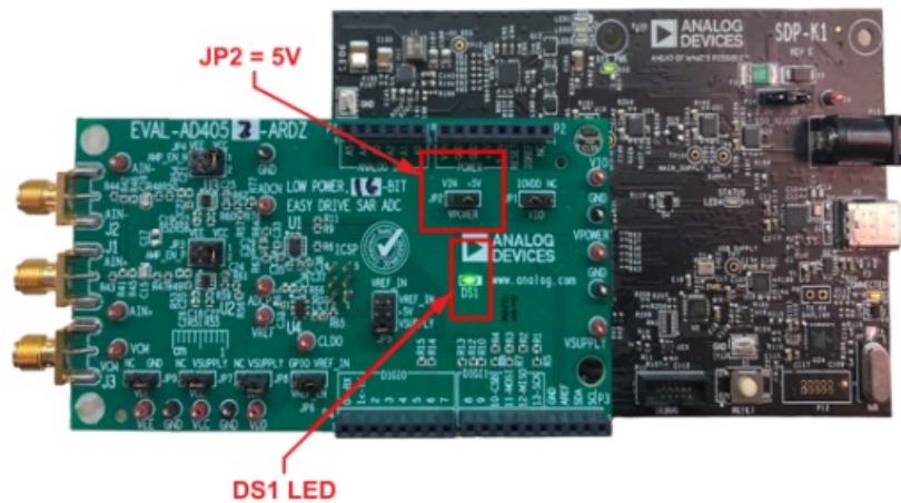
Figure 4. EVAL-AD4052-ARDZ on USB Power
