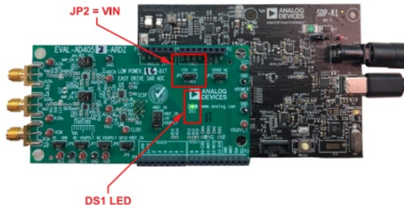
Figure 5. EVAL-AD4052-ARDZ on DC Jack Power
