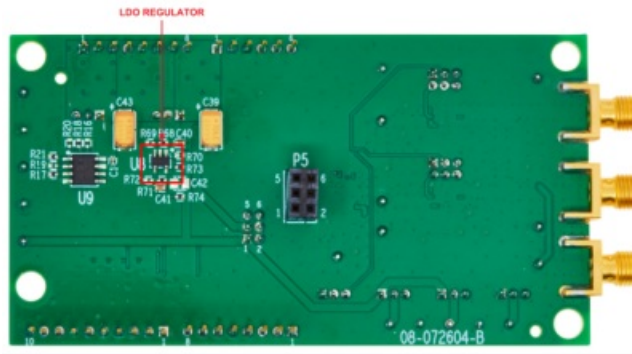
Figure 9. EVAL-AD4052-ARDZ Evaluation Board Circuitry Locations Bottom Side
