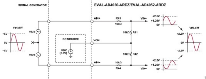
Figure 15. Floating Differential Signal Generator Example
