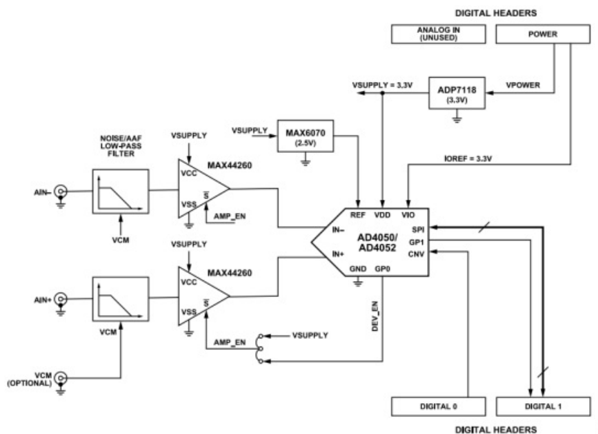
Figure 7. EVAL-AD4050-ARDZ/EVAL-AD4052-ARDZ Simplified Block Diagram
